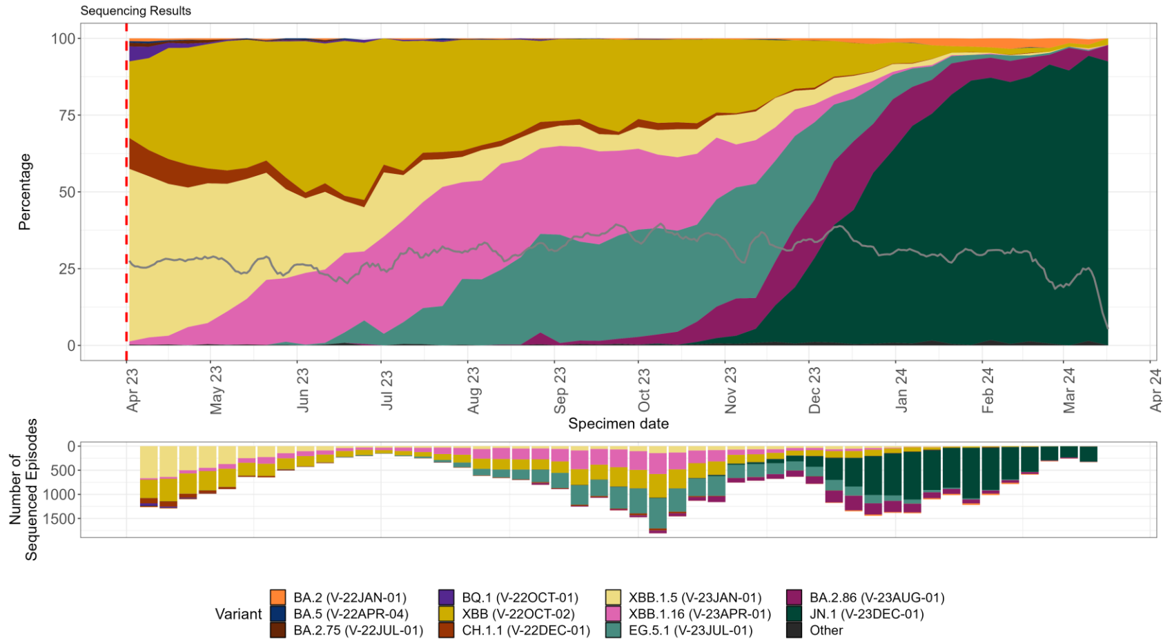
Figure 13. Prevalence of SARS-CoV-2 variants amongst available sequenced cases for England from 2 April 2023 to 17 March 2024 [note 6]
