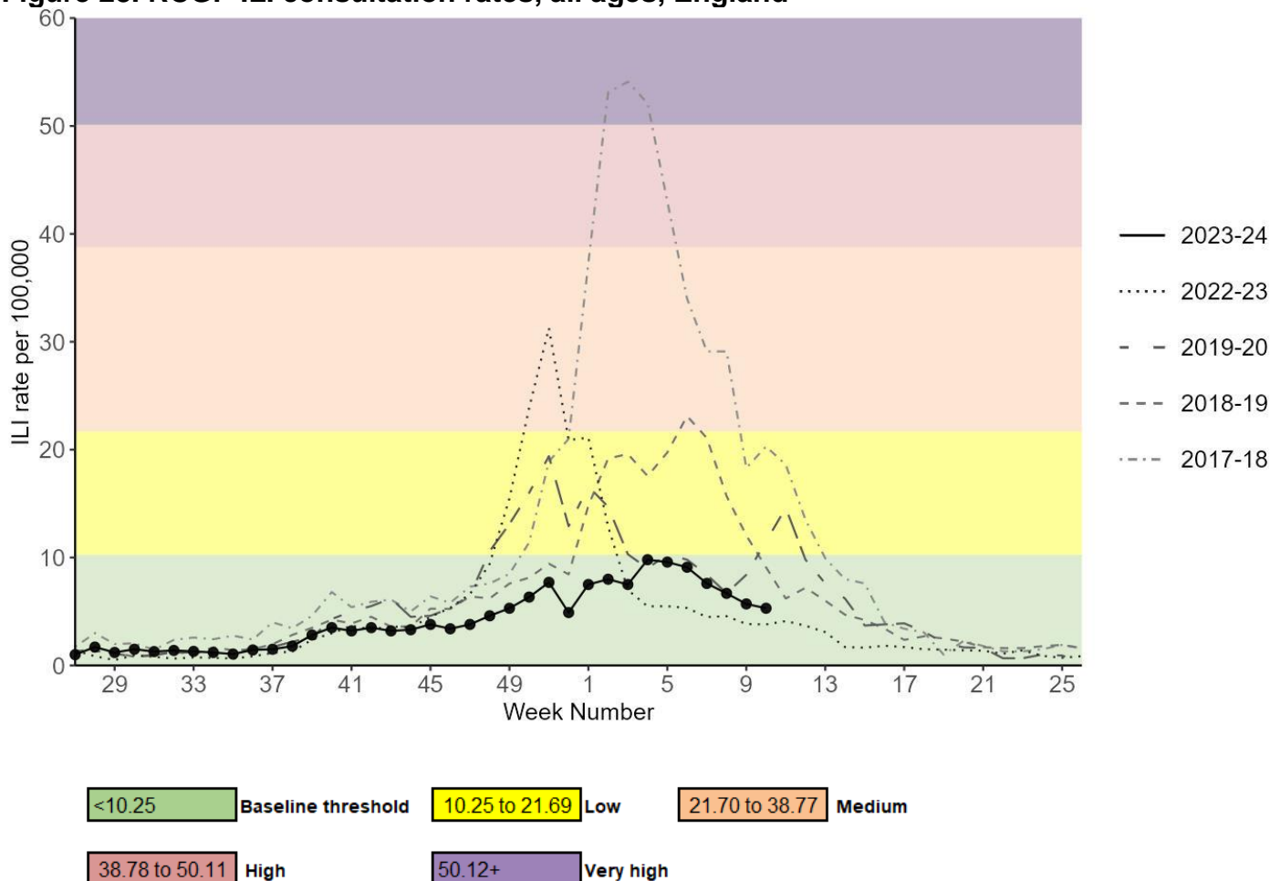
Figure 28. RCGP ILI consultation rates, all ages, England
