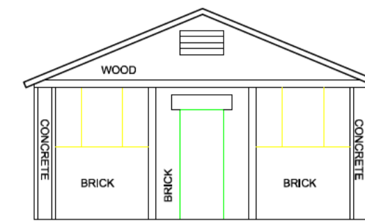
SOUTH ELEVATION BUILDING 4
