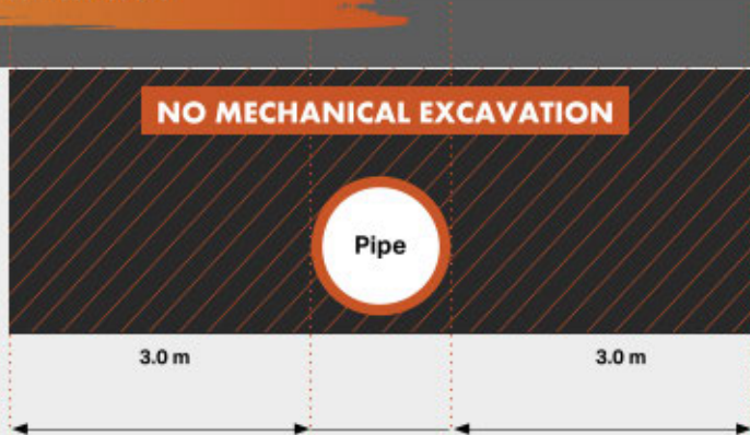
Figure 1. Excavation restrictions
