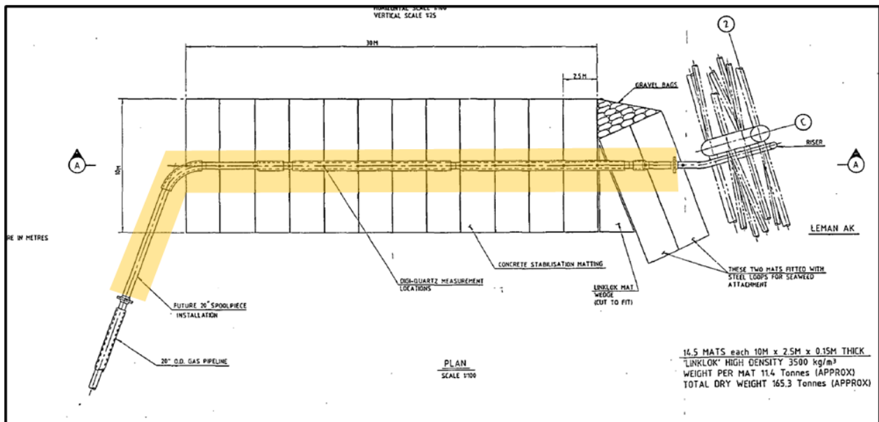
Figure 5-4 – Assumed PL363 spool removal at Leman F
