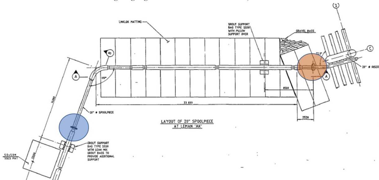
Figure 5-3 – Scope 3 disconnection options at Lemna A
