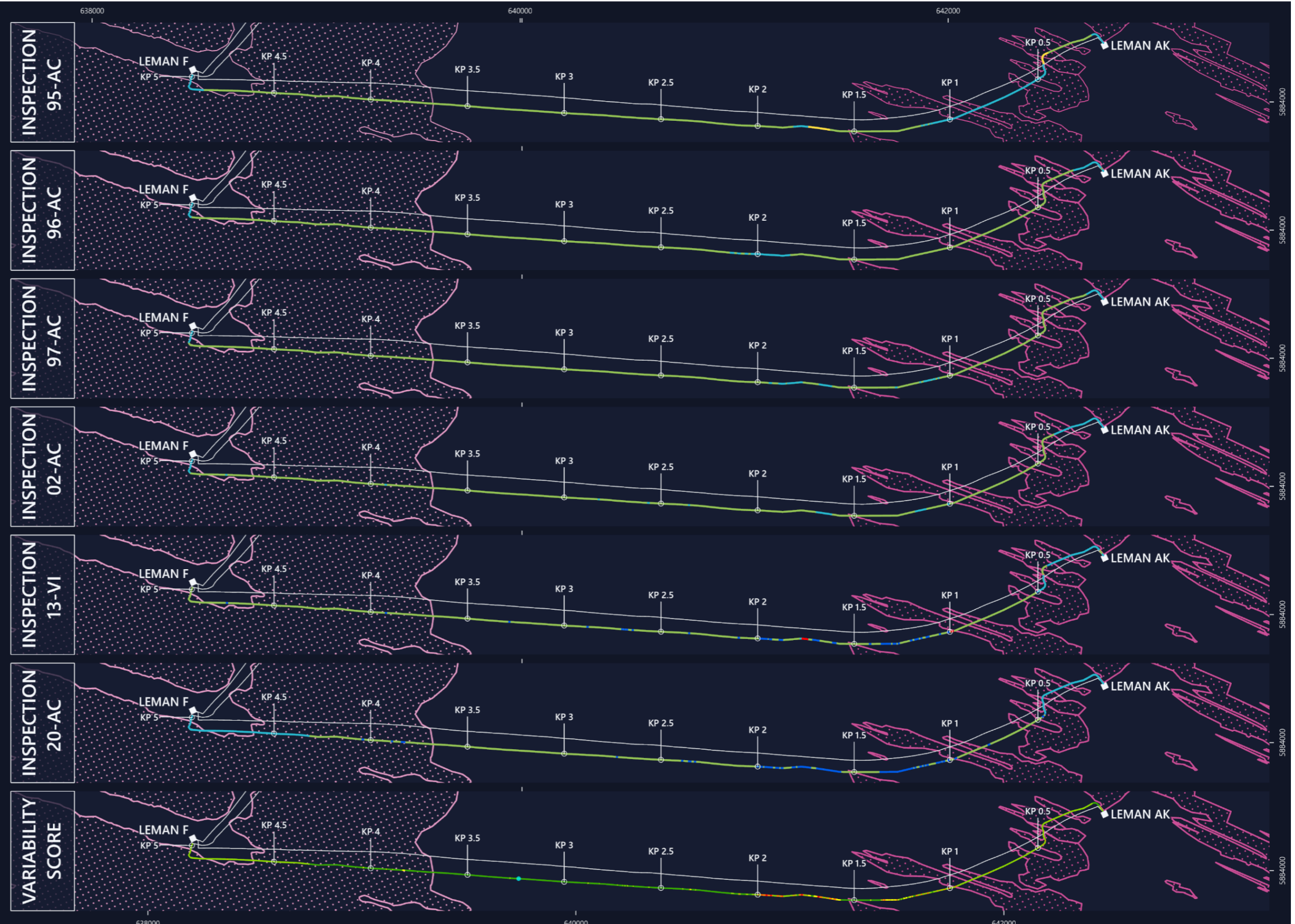
Figure 7-9 – Leman F Power Cable Historical Spanogram Results (S0806 / PL5148)
