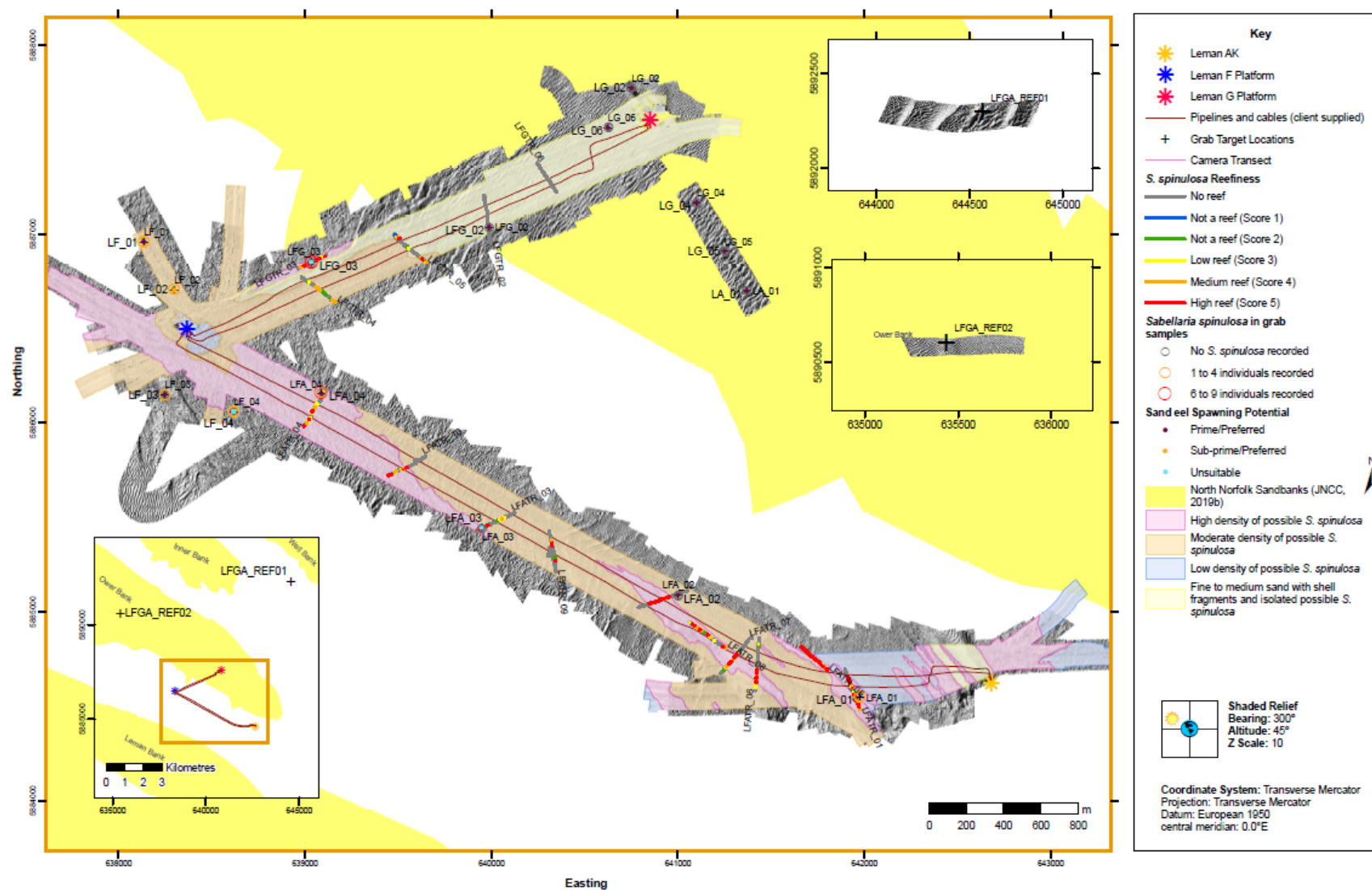
Figure 2-2 – Leman F &amp; G Layout, Overlaid with reef density and sandeel habitat
