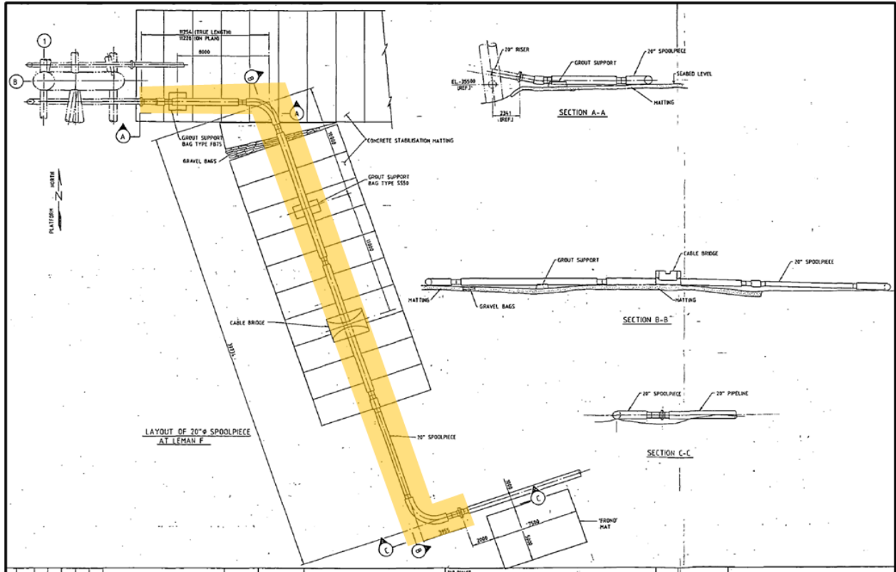
Figure 5-5 – Assumed PL363 spool removal at Leman F
