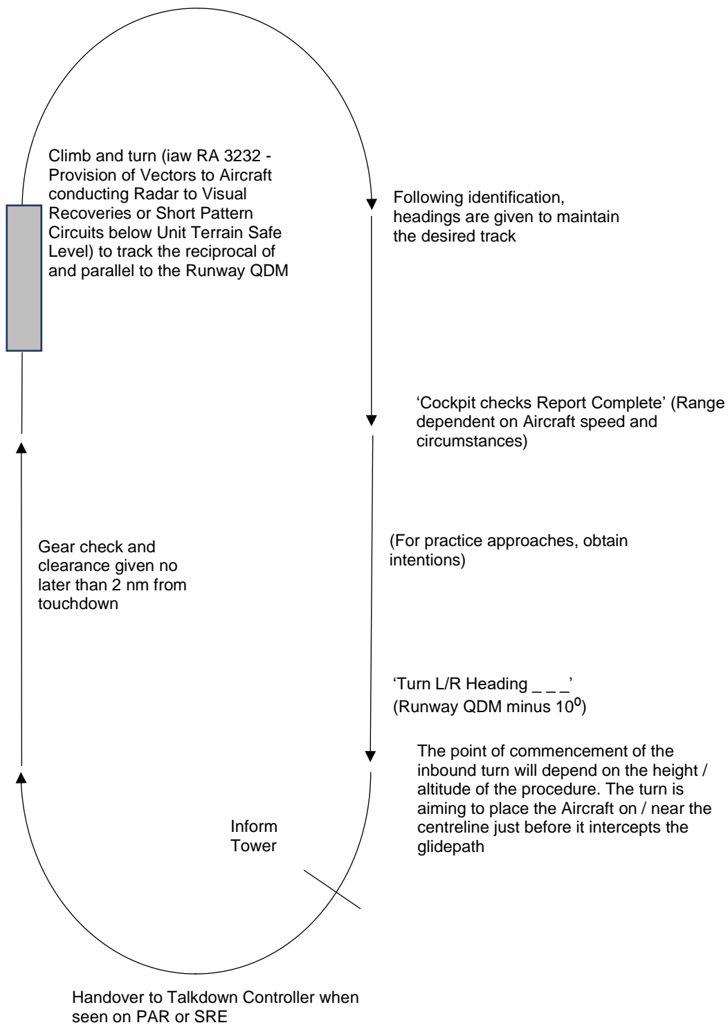
Figure 3: Director Procedures – Short Pattern Circuit
