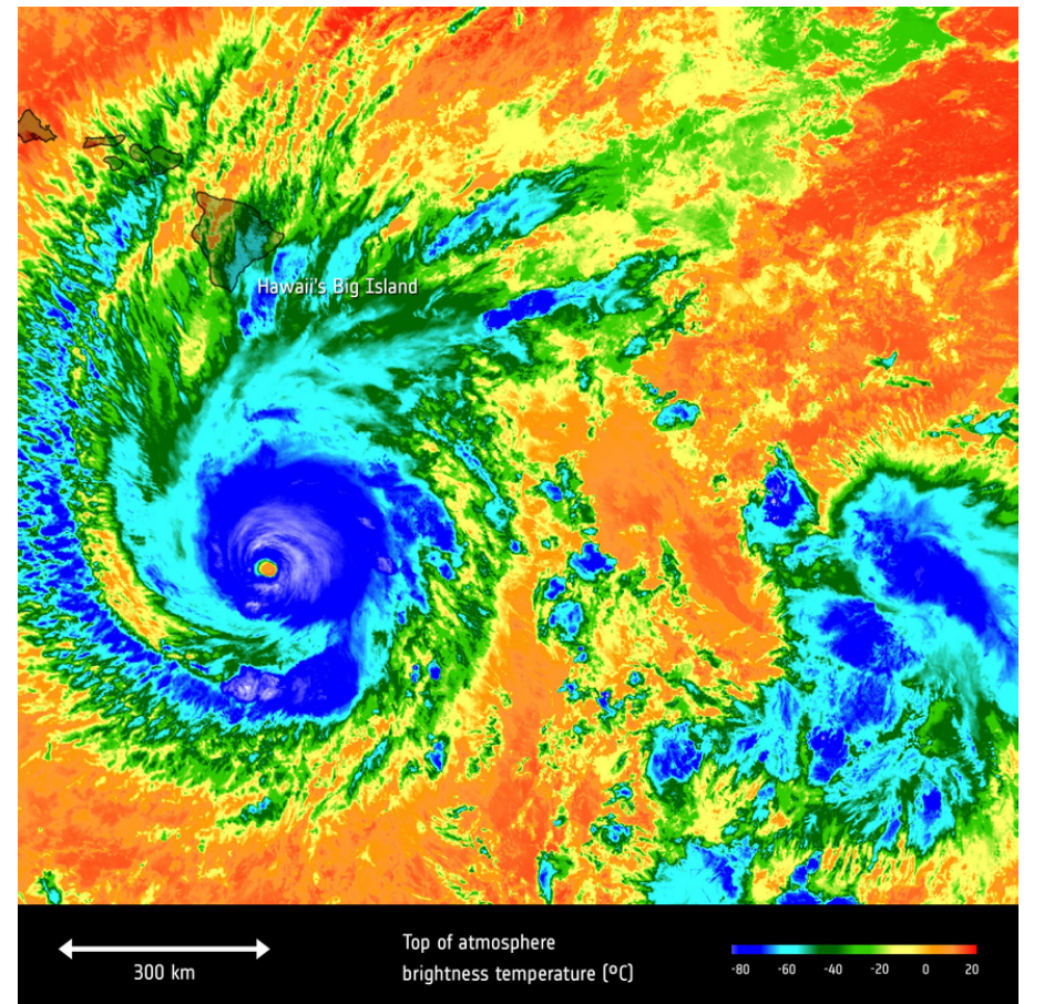
Hurricane Lane temperature
