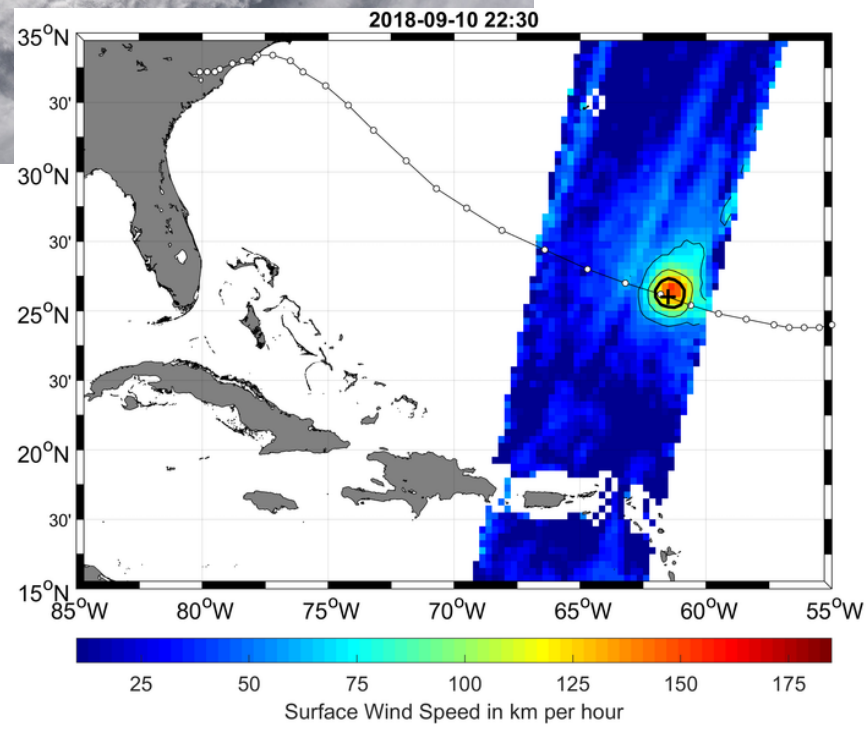
Hurricane Florence wind speed
