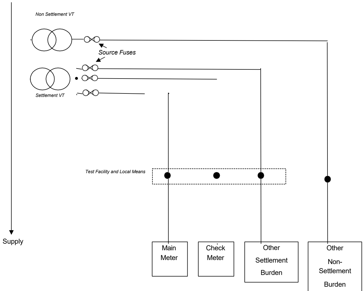
Figure 1: Fusing arrangements for cable runs of more than 30 metres distance between source fusing and local means of isolation 41 4243 .
