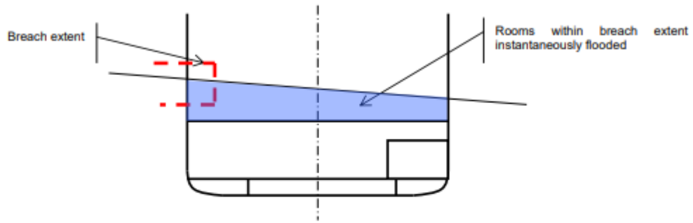
Stage 1: Downflooding through non-watertight deck
