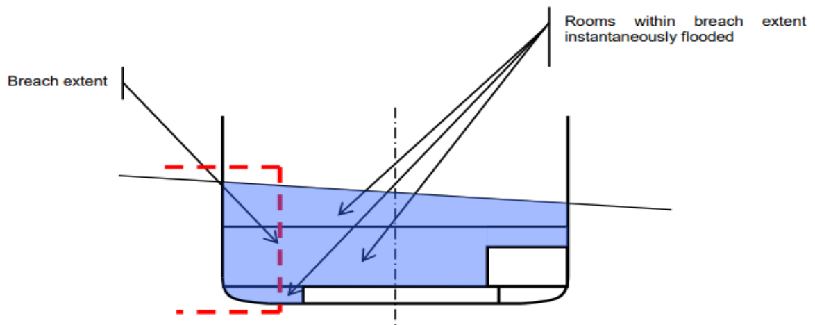
Stage 1: Cross-flooding of opposite room
