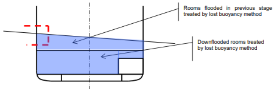
Final (full) phase of stage 1
