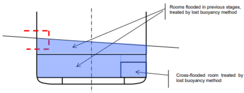
Full (final) phase of stage 2
