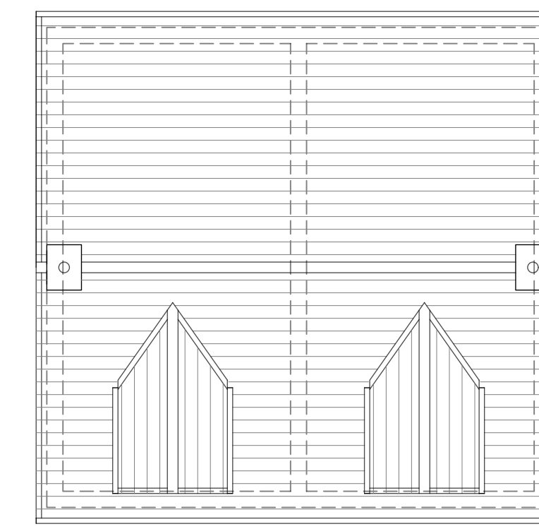
Roof Plan - Parham
