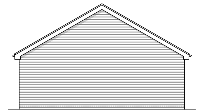
Gable Elevation
