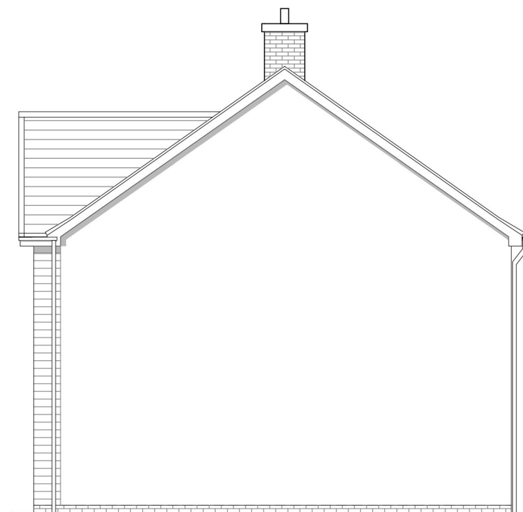
Gable Elevation
