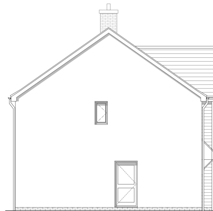
Gable Elevation
