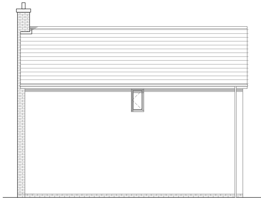
Gable Elevation
