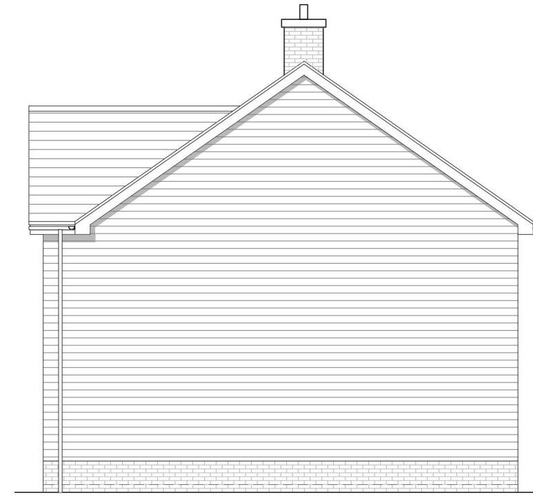
Gable Elevation
