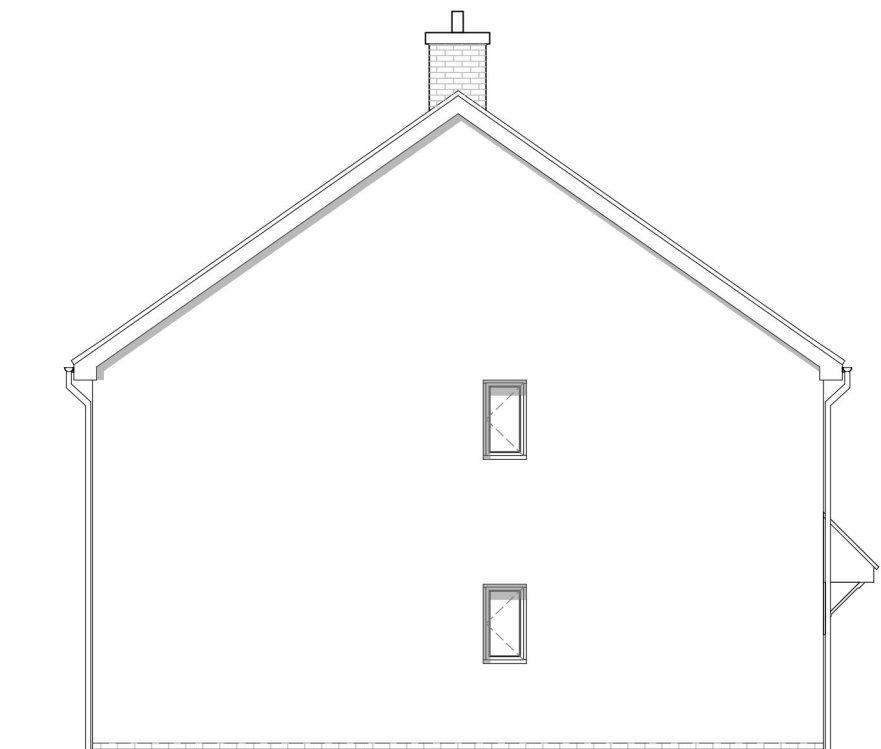
Gable Elevation
