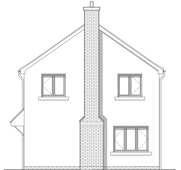
Active Gable Elevation
