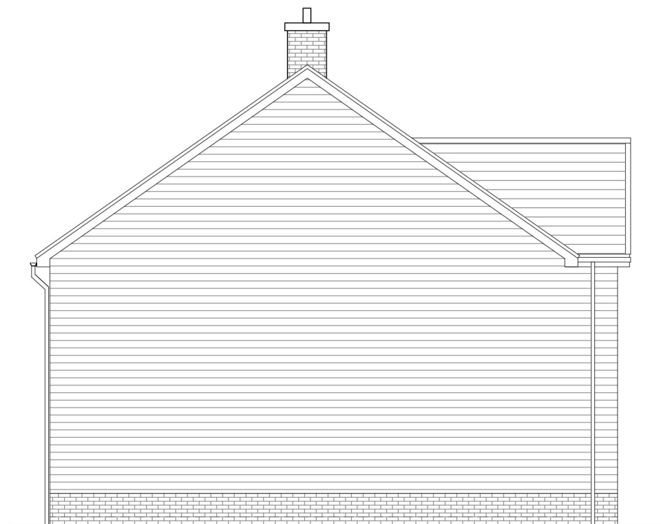
Gable Elevation
