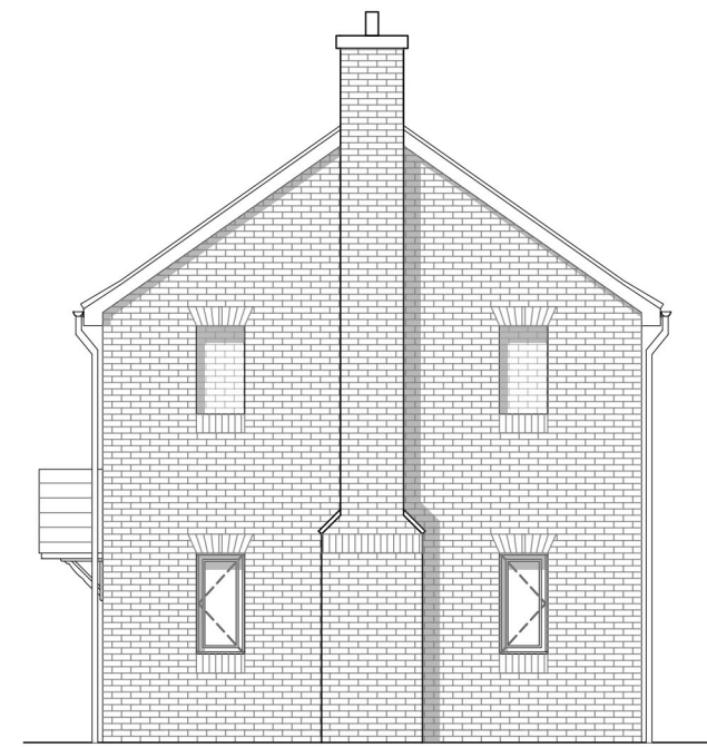
Active Gable Elevation
