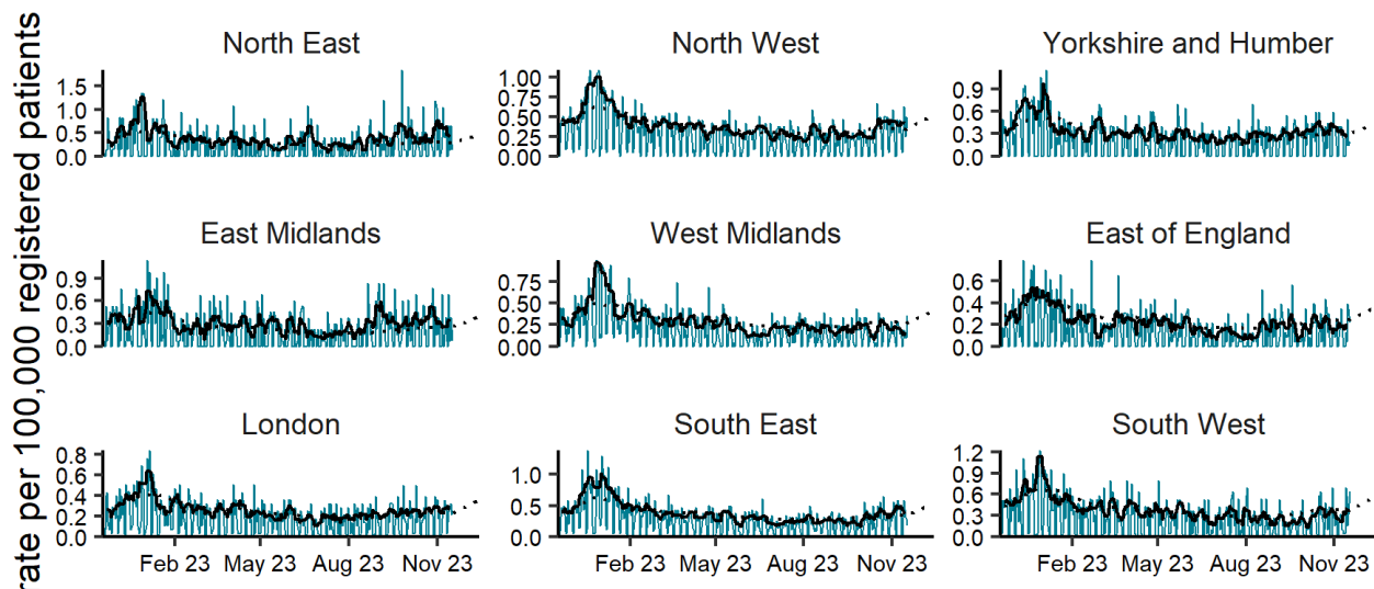
GP in-hours (combined): pneumonia by UKHSA region 18/11/2022 to 17/11/2023
