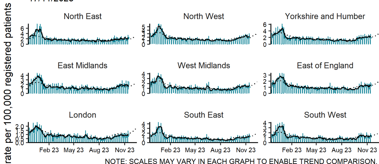
GP in-hours (combined): acute presenting asthma by UKHSA region 18/11/2022 to 17/11/2023
