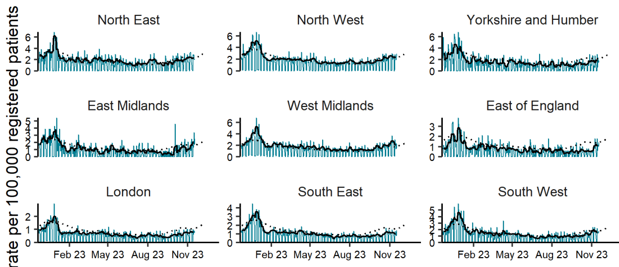
GP in-hours (Orchid): acute bronchitis by UKHSA region 21/11/2022 to 17/11/2023
