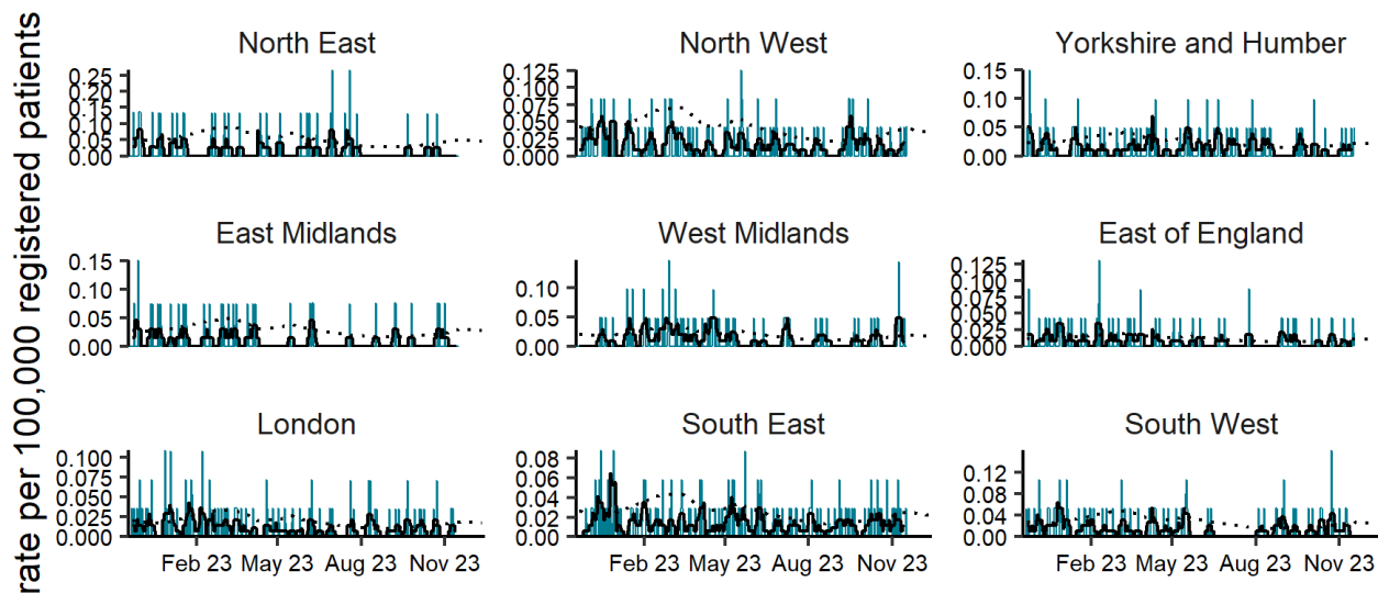
GP in-hours (combined): mumps by UKHSA region 18/11/2022 to 17/11/2023
