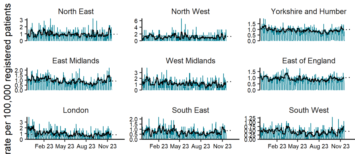
GP in-hours (TPP): vomiting by UKHSA region 20/11/2022 to 19/11/2023
