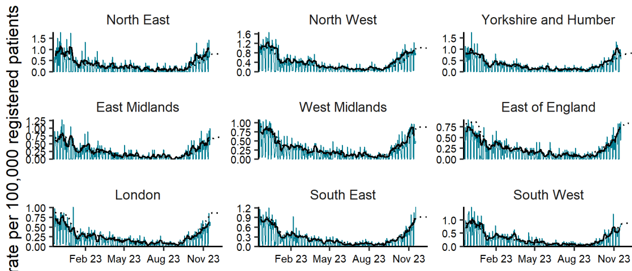
GP in-hours (combined): bronchiolitis by UKHSA region 18/11/2022 to 17/11/2023
