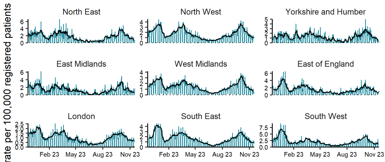
GP in-hours (Orchid): covid-19-like by UKHSA region 21/11/2022 to 17/11/2023
