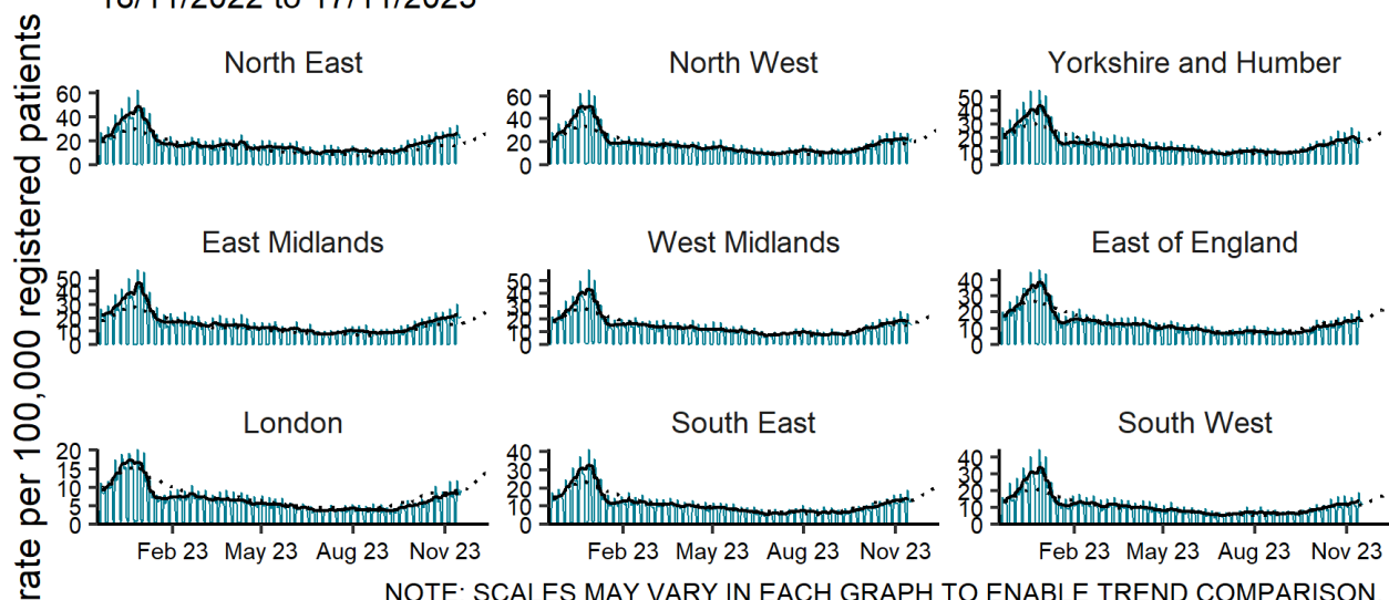
GP in-hours (combined): lower respiratory tract infection by UKHSA region 18/11/2022 to 17/11/2023
