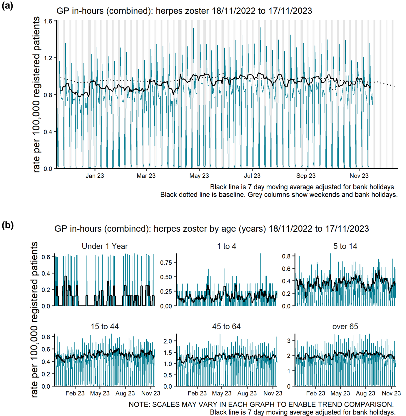
Figure 19: Daily incidence rate per 100,000 population (and 7-day moving average adjusted for bank holidays) for herpes zoster GP in hours consultations, England (a) nationally, (b) by age and (c) by UKHSA Region (population 18.8 million patients).
