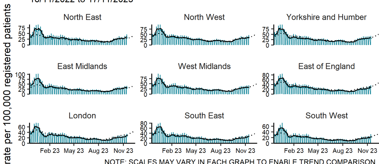
GP in-hours (combined): upper respiratory tract infection by UKHSA region 18/11/2022 to 17/11/2023
