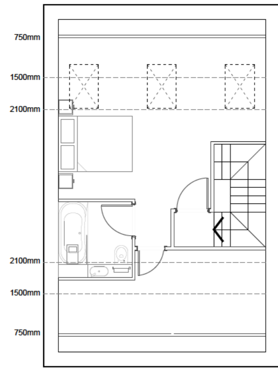
00 Proposed First Floor Plan
