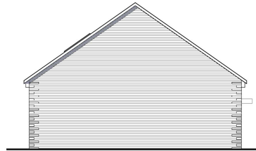
D Proposed Side Elevation
