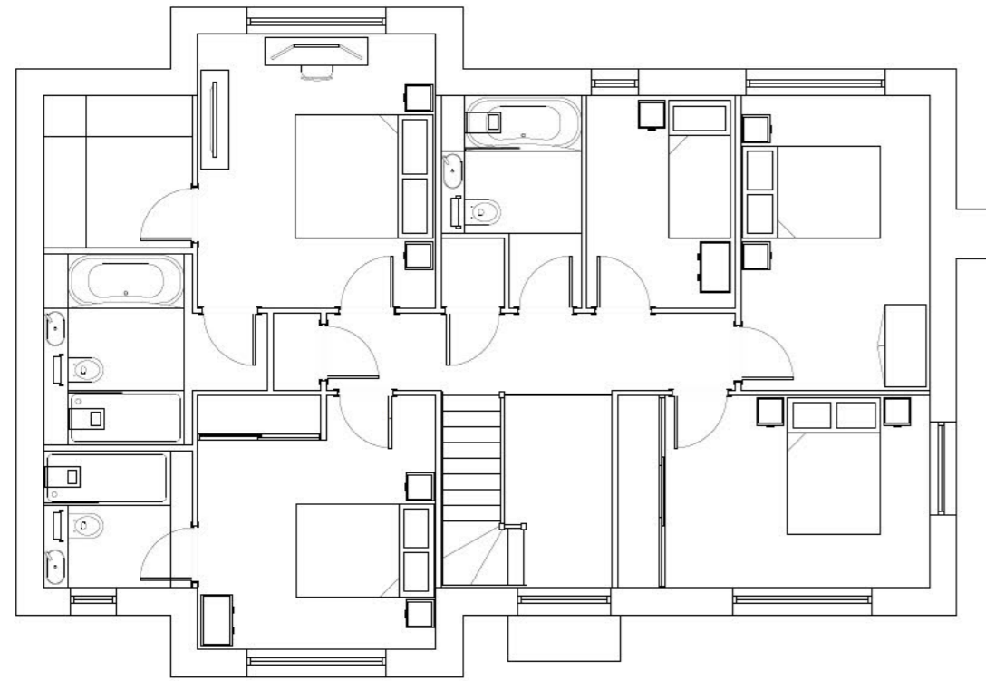
01 Proposed First Floor Plan
