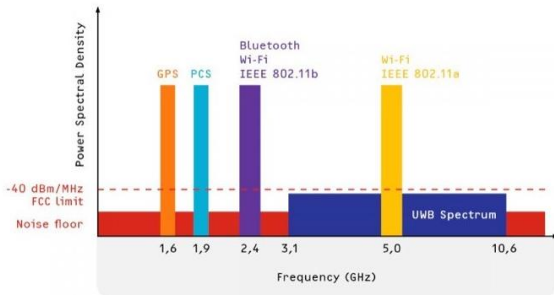
Figure 17 UWB spectrum
