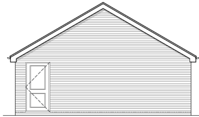
Gable Elevation
