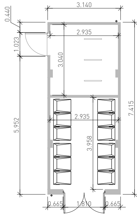
Floor Plan
