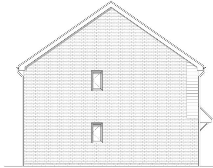
Gable Elevation
