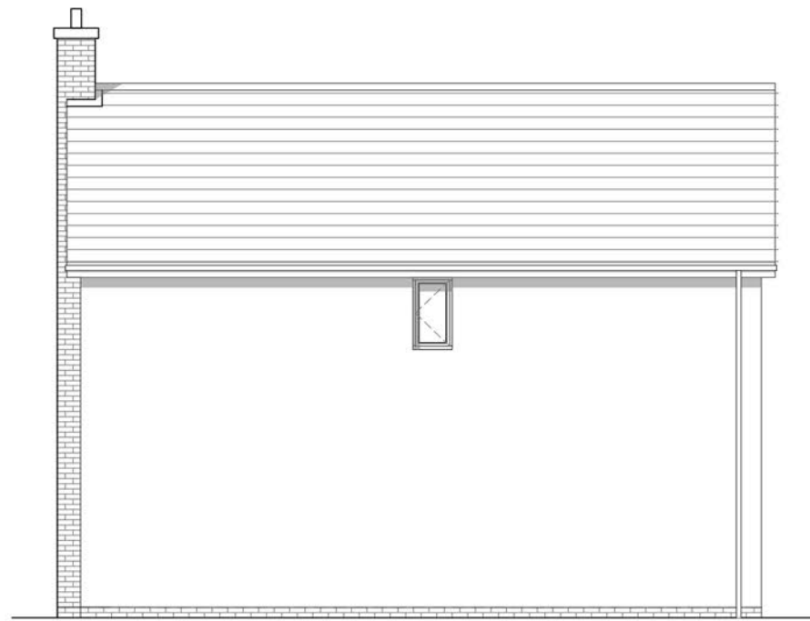
Gable Elevation
