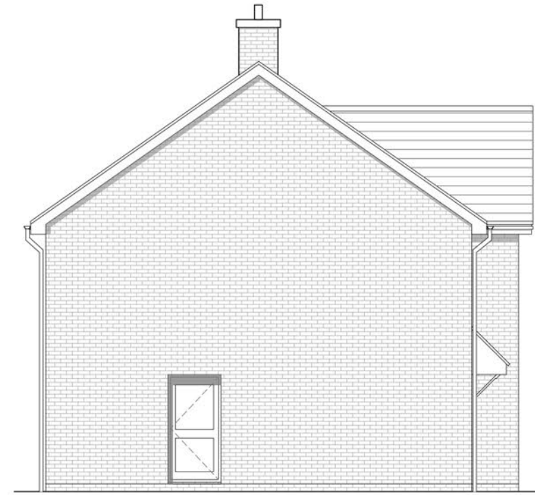
Gable Elevation
