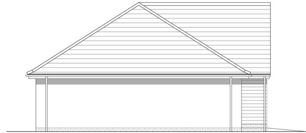
Gable Elevations
