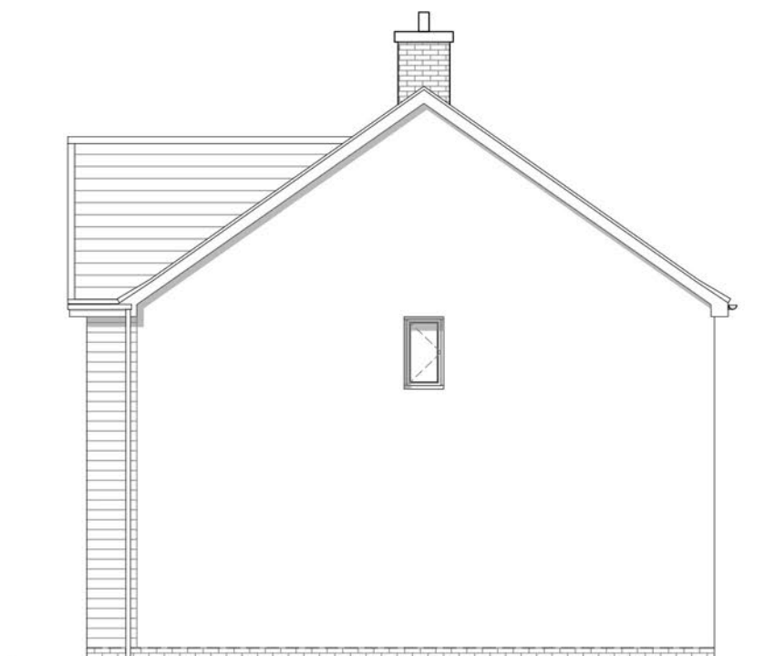
Gable Elevation
