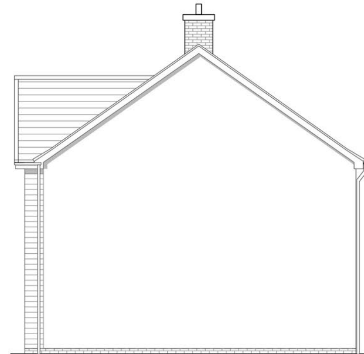
Gable Elevation
