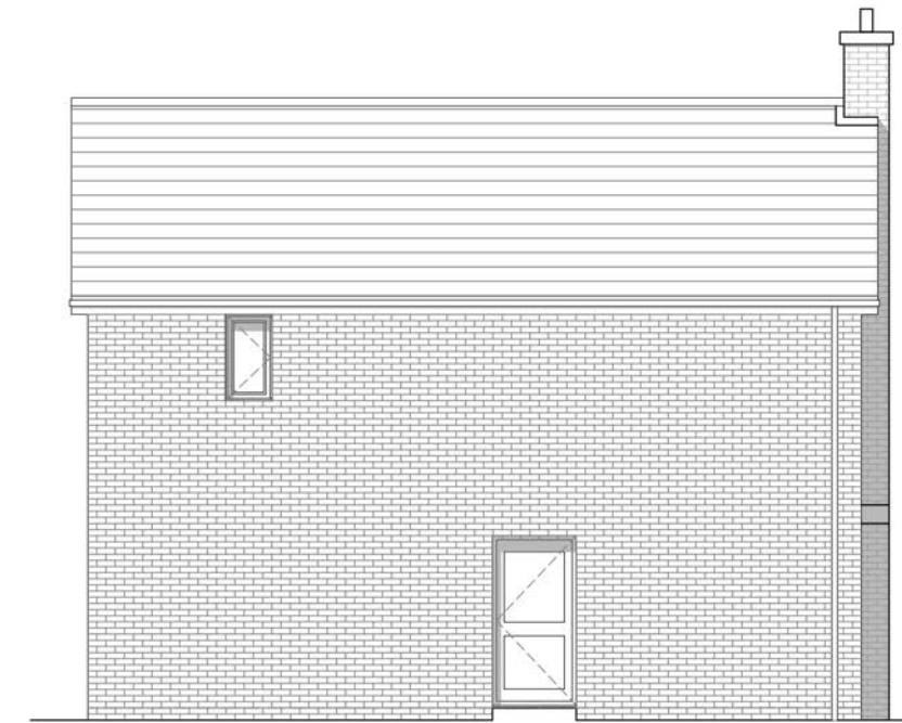
Gable Elevation
