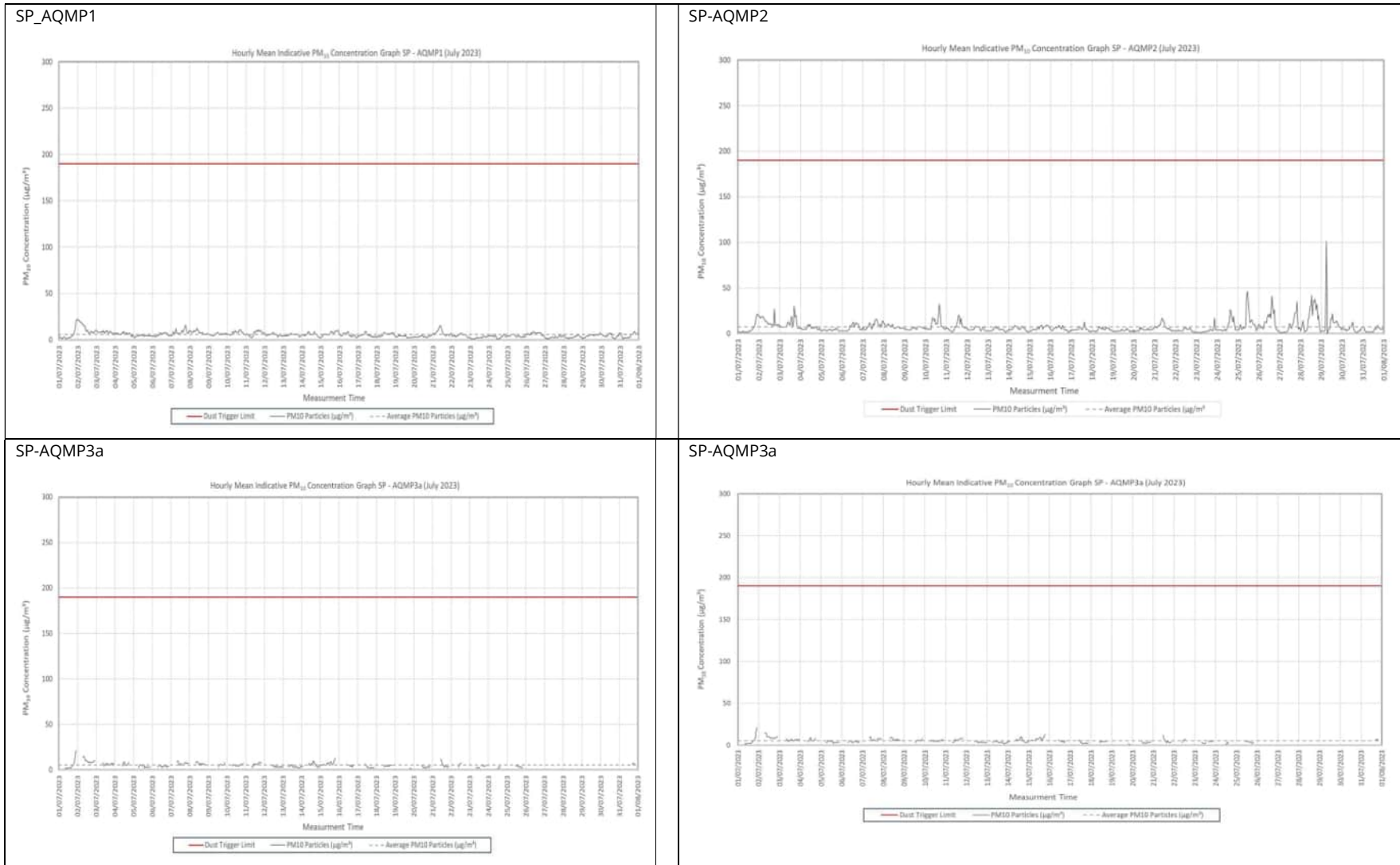
Figure 2: Continuous dust 1-hour mean indicative PM 10 concentration for SP-AQMP1 for July 2023
