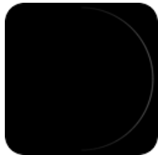
New Moon
