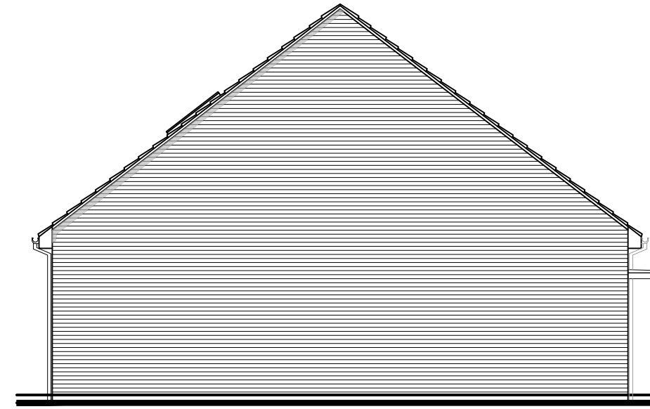
B Proposed Side Elevation
