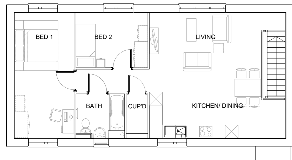
01 Proposed First Floor Plan
