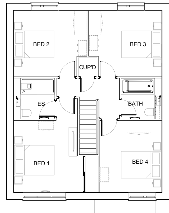
01 Proposed First Floor Plan
