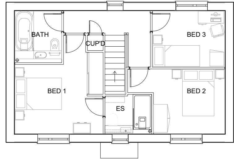
01 Proposed First Floor Plan
