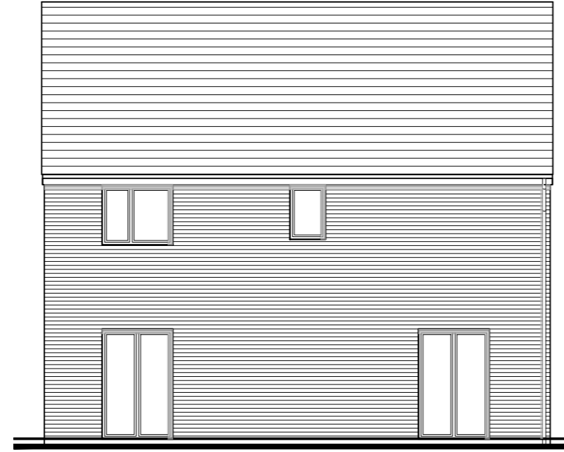
C Proposed Rear Elevation
