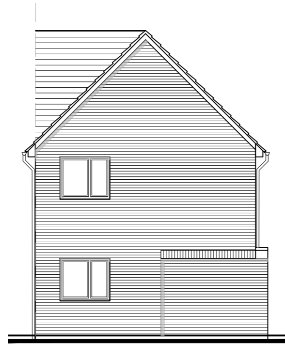
A Proposed Front Elevation
