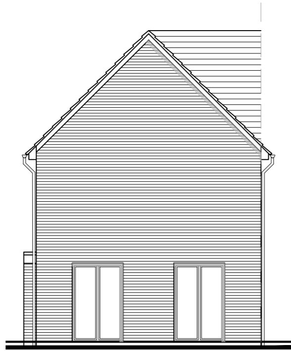
C Proposed Rear Elevation
