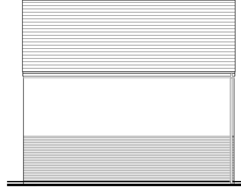
D Proposed Side Elevation
