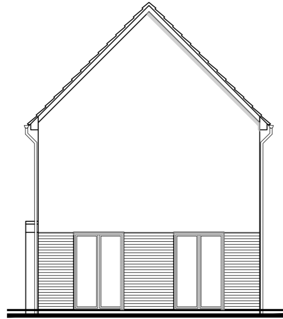
C Proposed Rear Elevation
