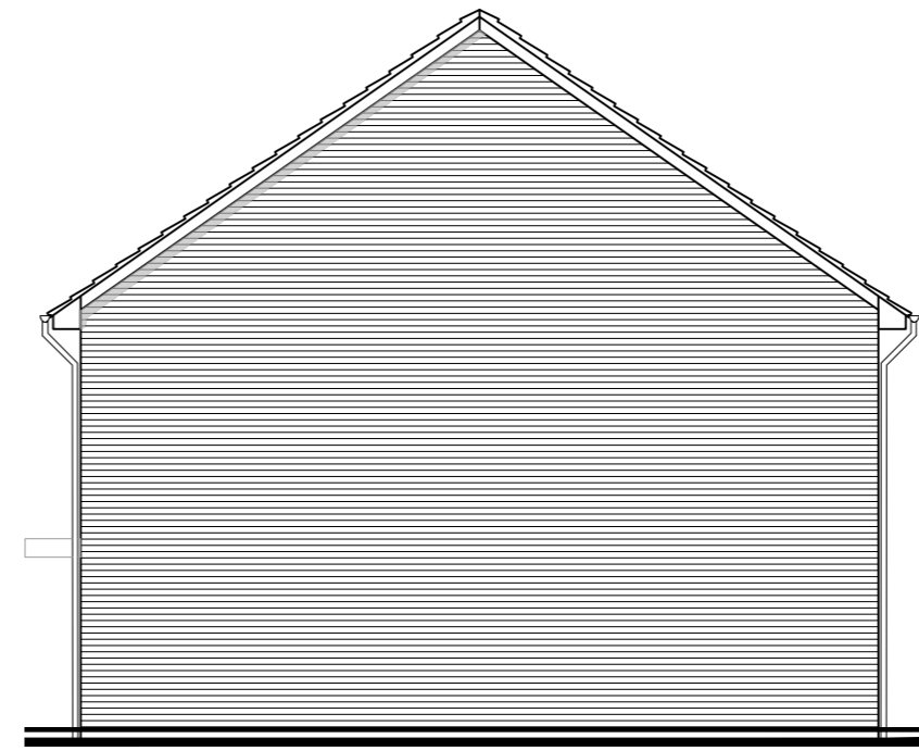
D Proposed Side Elevation Elevation to plots: 04, 16, 24, 31, 88
