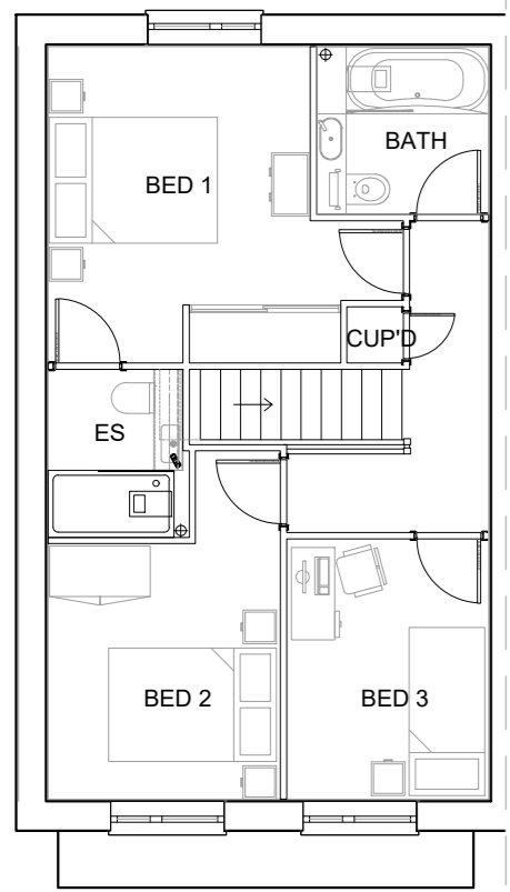
01 Proposed First Floor Plan
