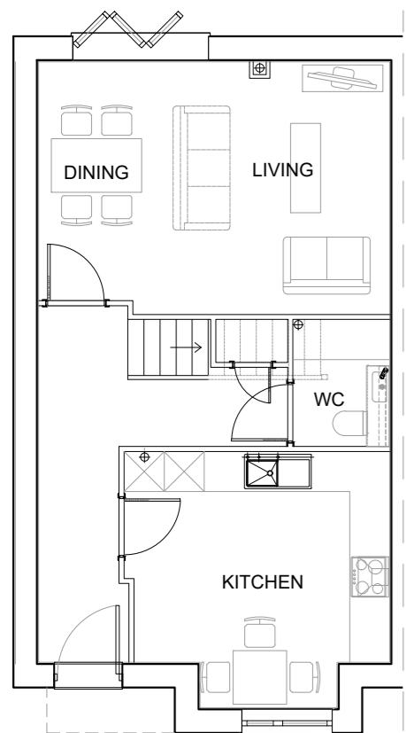
00 Proposed Ground Floor Plan
