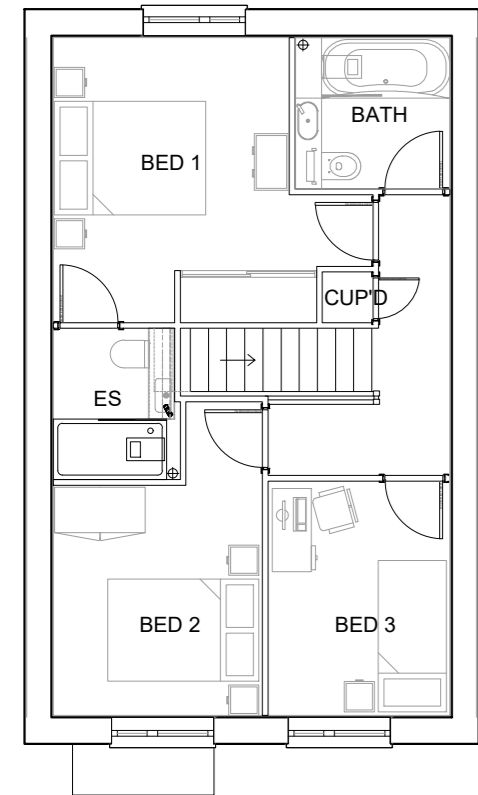
01 Proposed First Floor Plan
