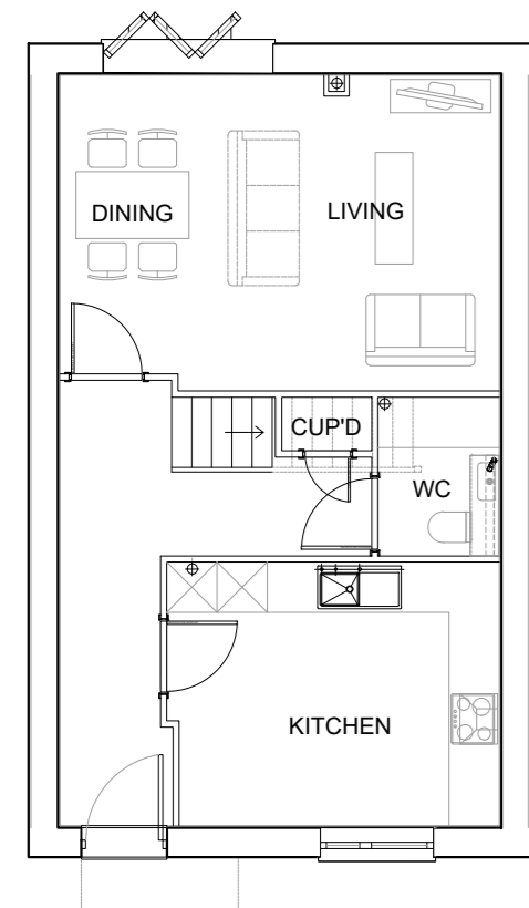
00 Proposed Ground Floor Plan
