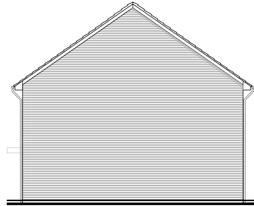
D Proposed Side Elevation To semi detached units: 01, 11, 14, 28, 36, 42, 91
