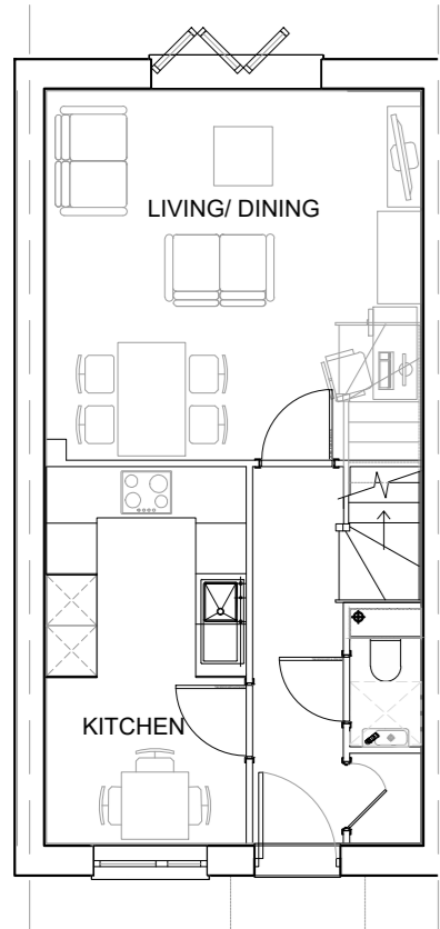
00 Proposed Ground Floor Plan
