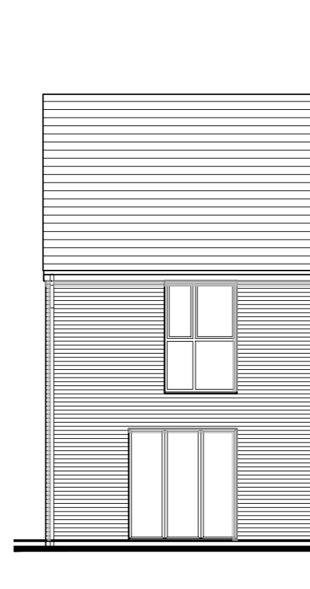
C Proposed Rear Elevation
