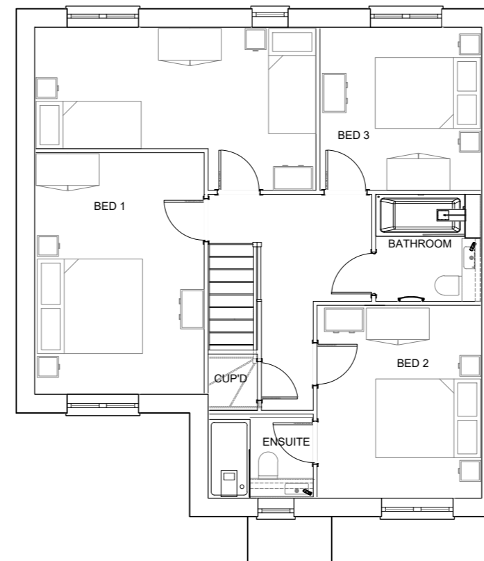
09 HA 4.02 Proposed First Floor Plan
