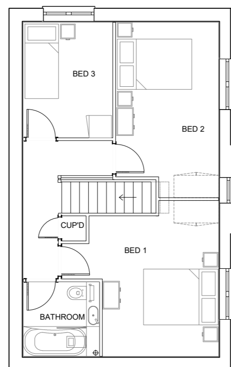
07 HA 3.05 Proposed First Floor Plan
