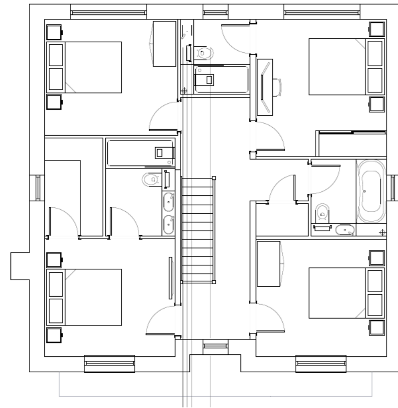
01 Proposed First Floor Plan
