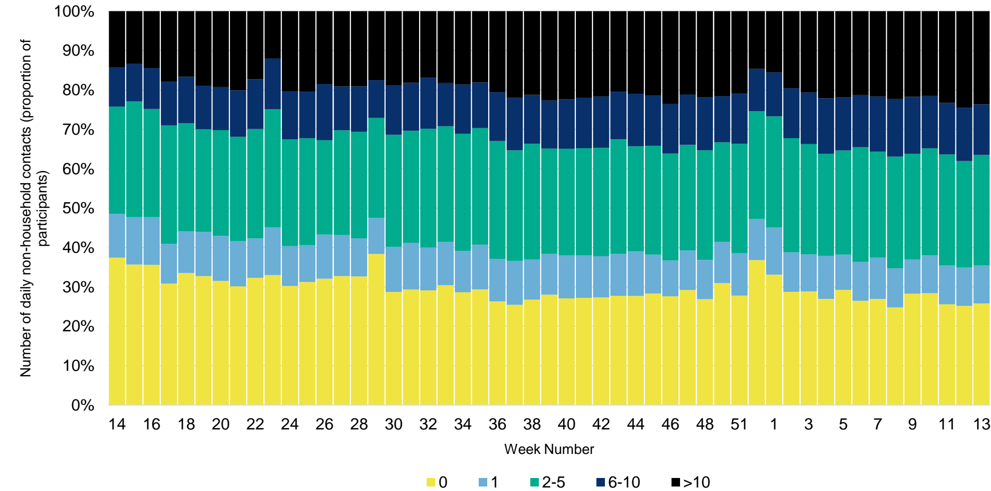
Figure 28: FluSurvey participants’ self-reported number of social contacts outside the household
