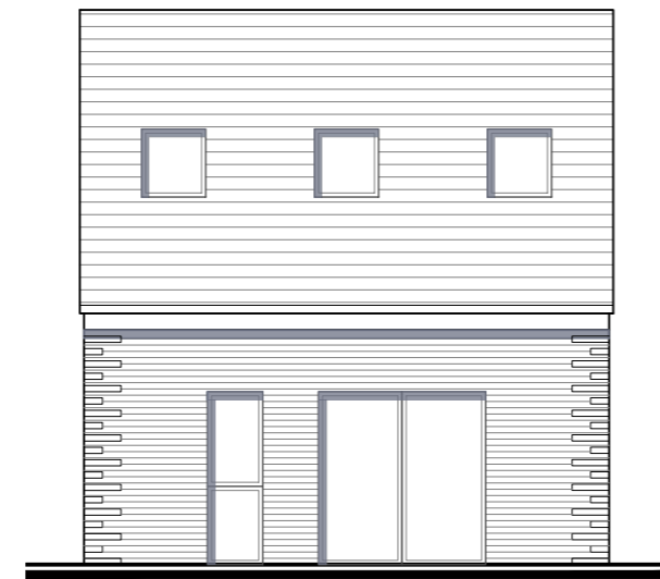
C Proposed Rear Elevation
