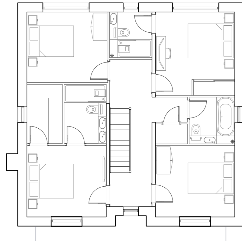
01 Proposed First Floor Plan
