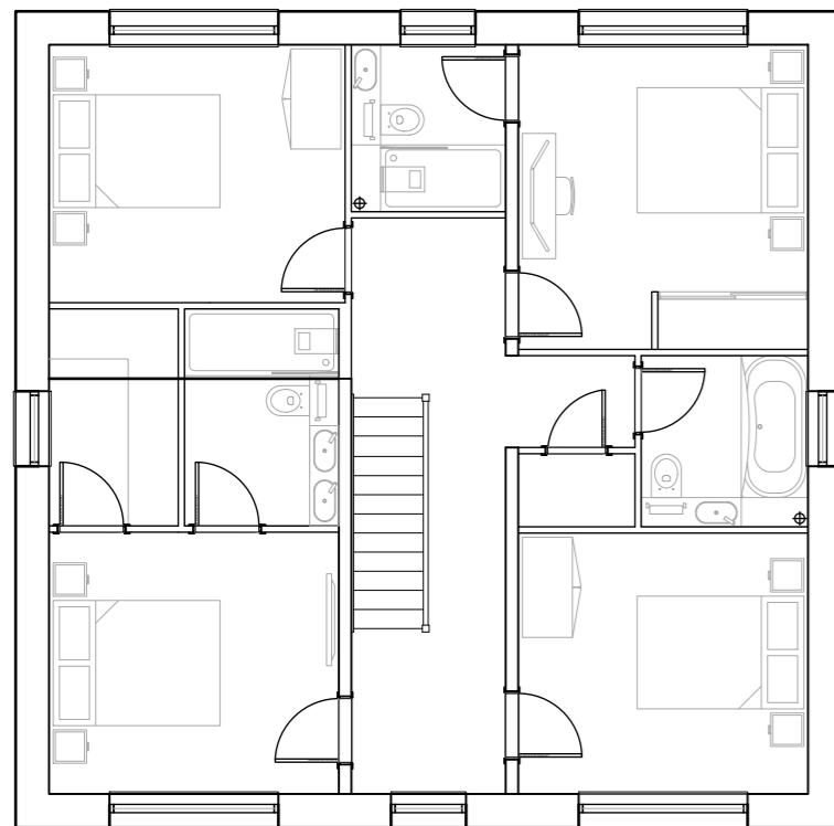
01 Proposed First Floor Plan
