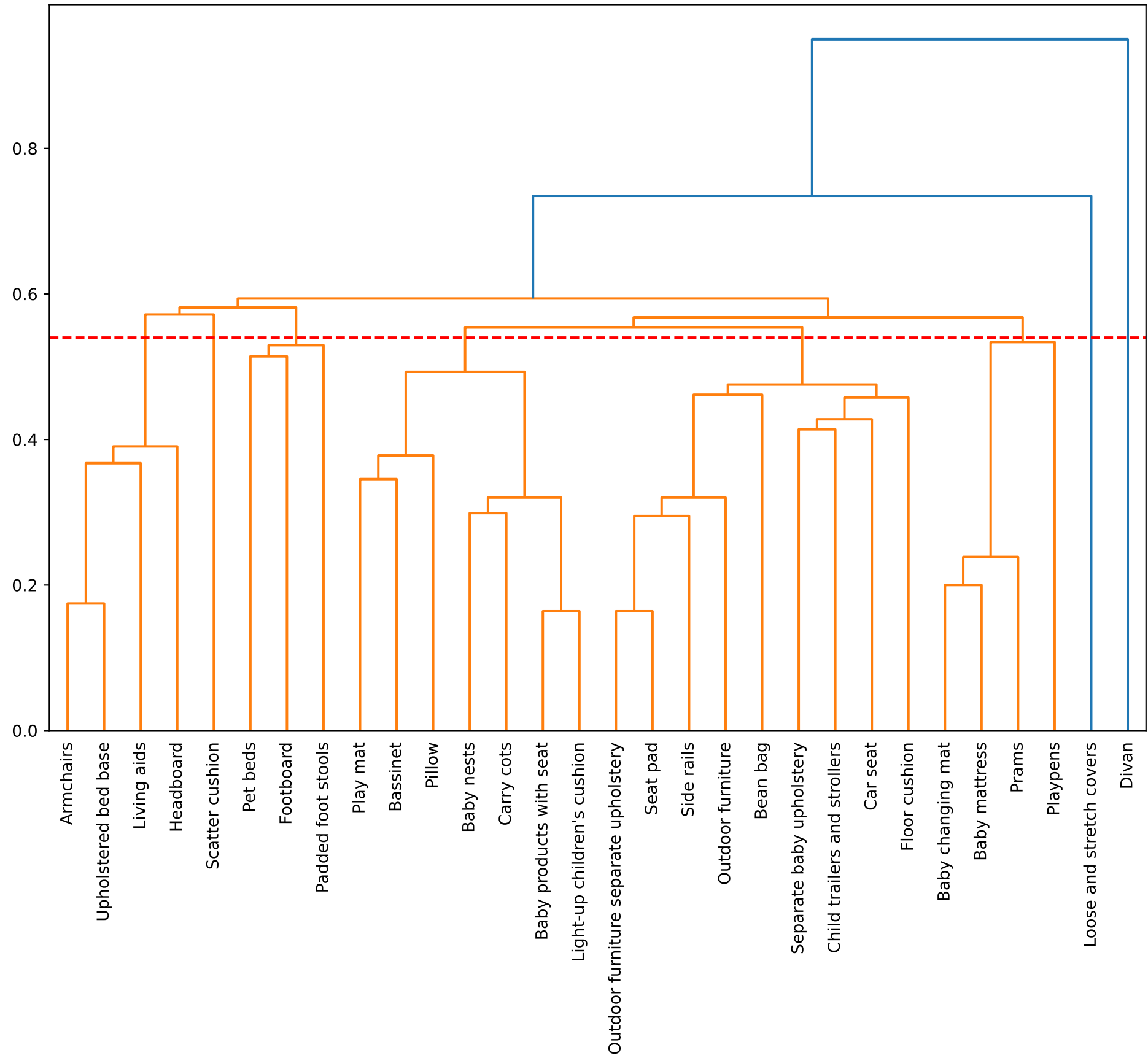
Similarity Dendrogram (Injury, Damage, Exposure; Euclidean Distance)
