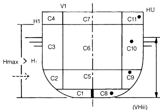
FIG A-11 INTERPRETATION OF COMBINED LONGITUDINAL & HORIZONTAL SUBDIVISION
