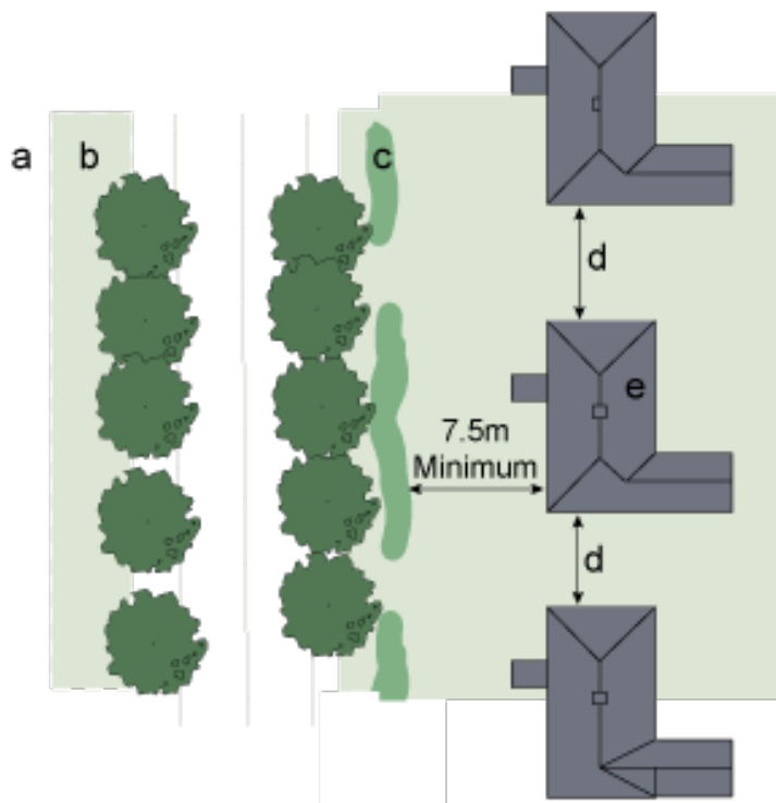
a. Footway b. Verge c. Hedge d. Distance not less than half width of house e. Varied houses
