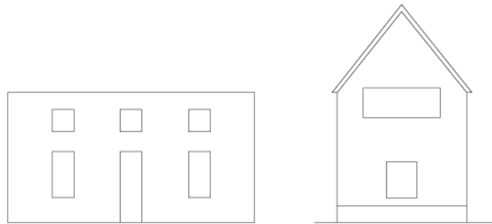
(Left) Vertically proportioned openings used with square openings to balance a horizontal elevation. (Right) Horizontally proportioned opening balances a vertical projecting wing
