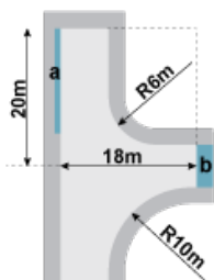
Size 2, Side Turn
