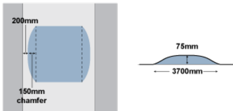
(Left) Plan view (Right) Section along road
