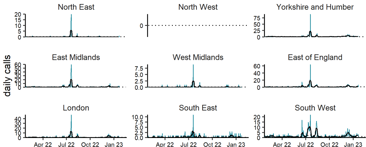
NASSS: impact of heat or cold by region 23/01/2022 to 22/01/2023
