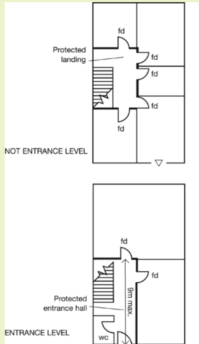
Figure 7 – Multi-storey flat with protected entrance hall and landing
