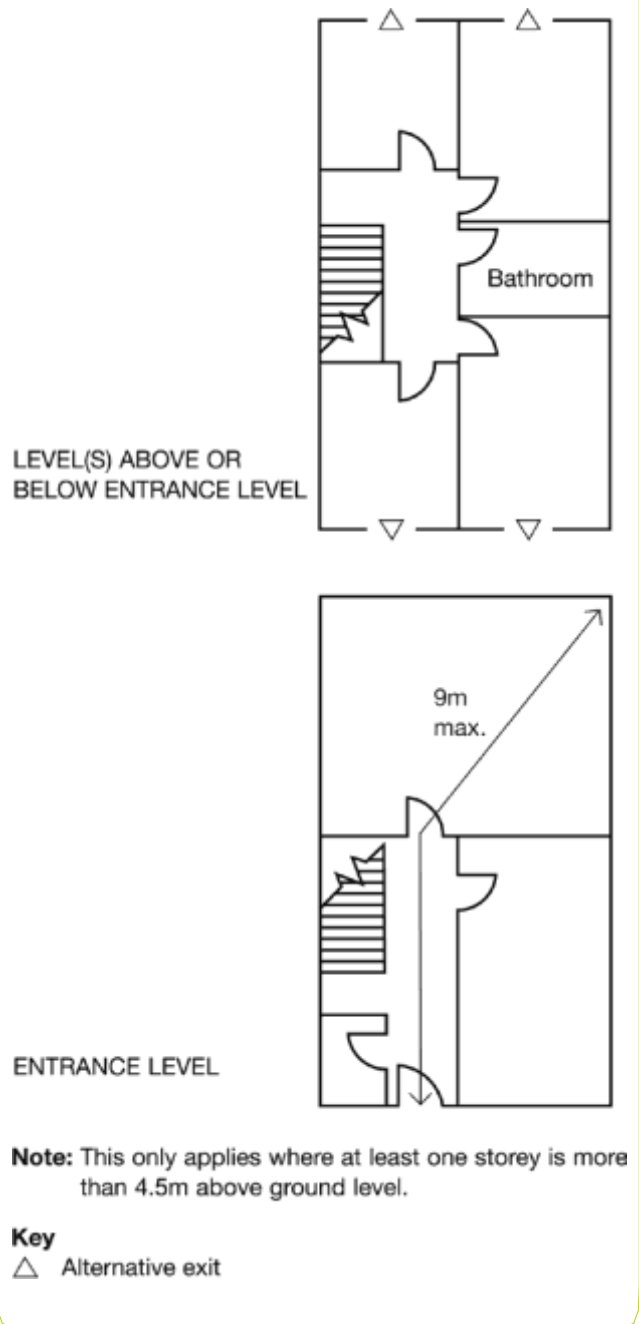
Figure 6 – Multi storey flat with alternative exits, from each habitable room, except at entrance level
