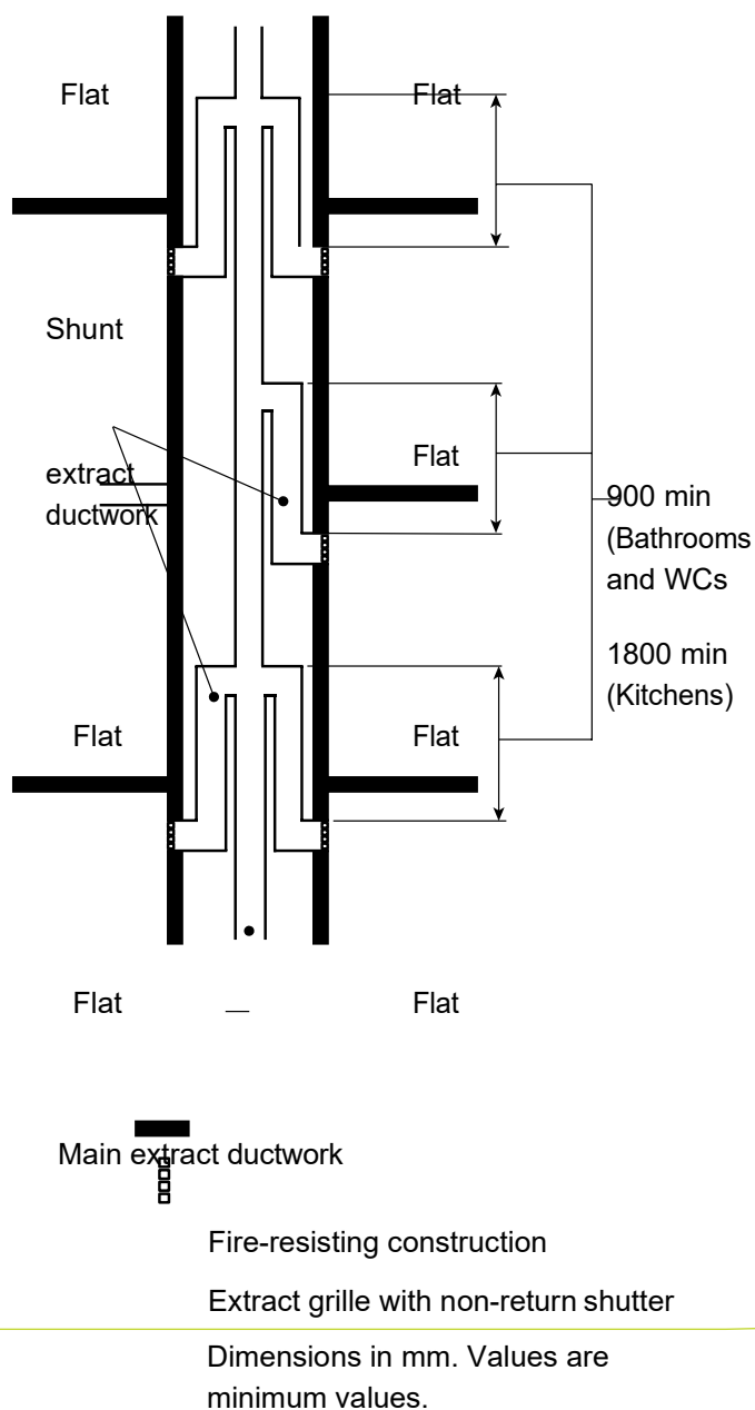
Figure 1 – Shunt duct arrangements
