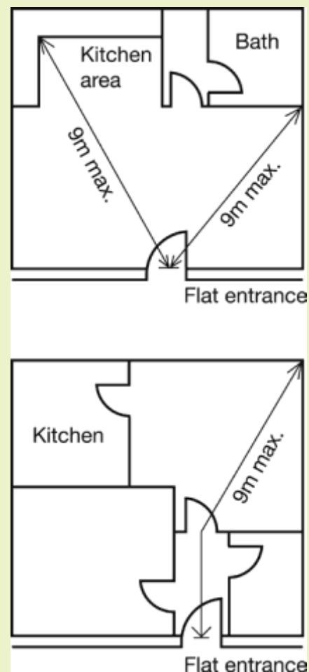
Figure 3 – Flat with limited travel distance
