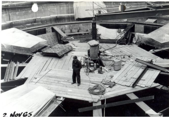
Photographs 12 & 13 - Wylfa during construction circa 1965
