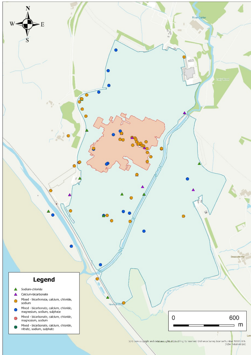
Figure 8. Groundwater types identified
