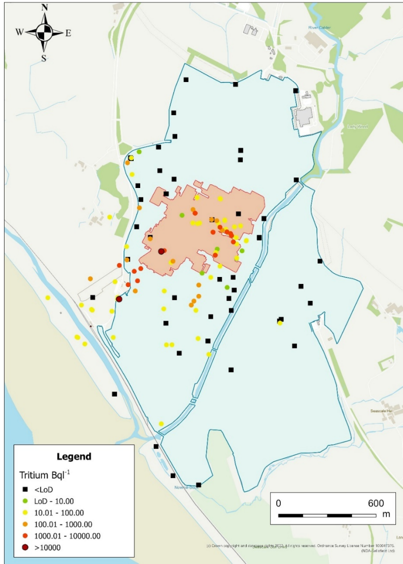
Figure 6. Average tritium concentrations (Bq l -1 )
