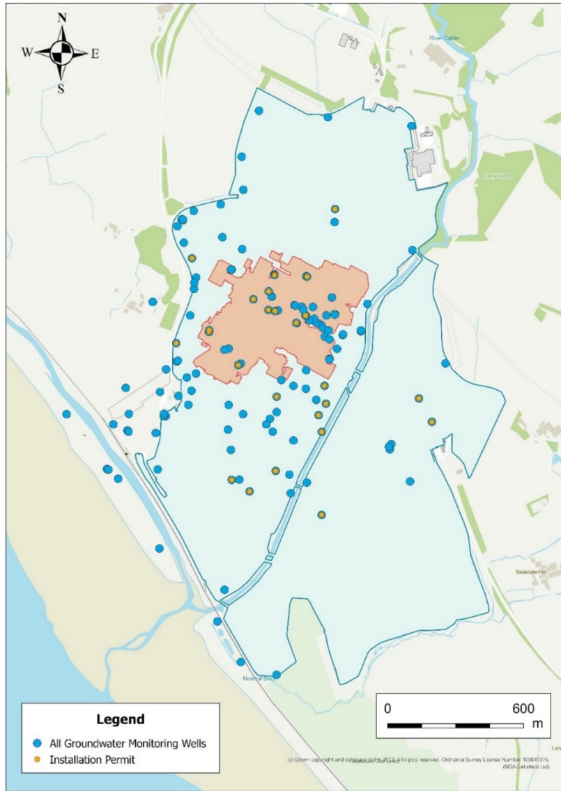
Figure 2. Groundwater Monitoring Network
