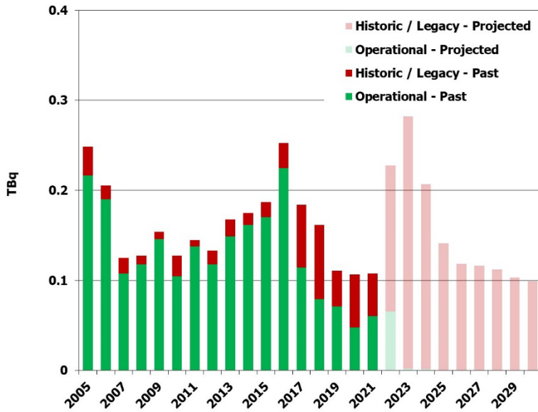
Figure 2. Past and projected total beta (excluding tritium) discharges from liquid effluents
