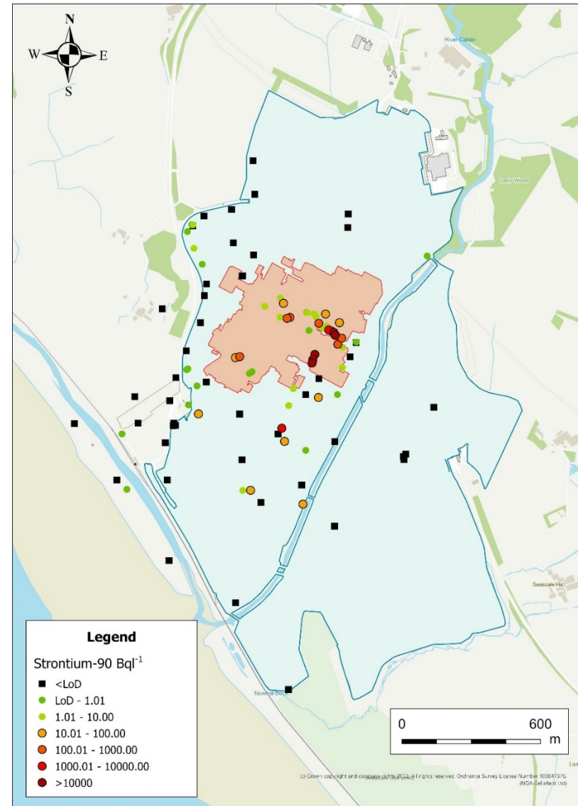
Figure 5. Average strontium-90 concentrations (Bq l -1 )
