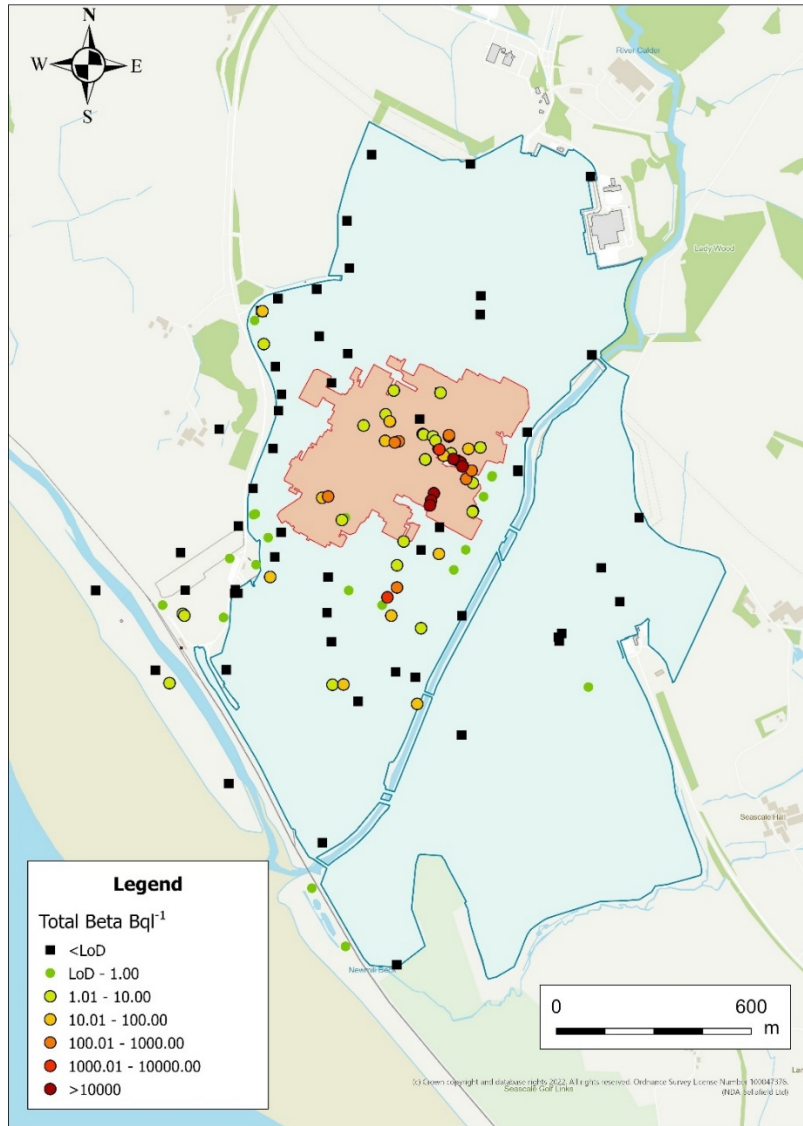
Figure 4. Average Total Beta concentrations (Bq l -1 )
