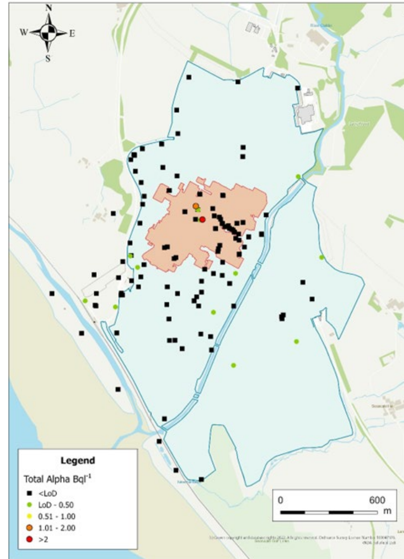
Figure 3. Average Total Alpha Concentrations (Bq l -1 )
