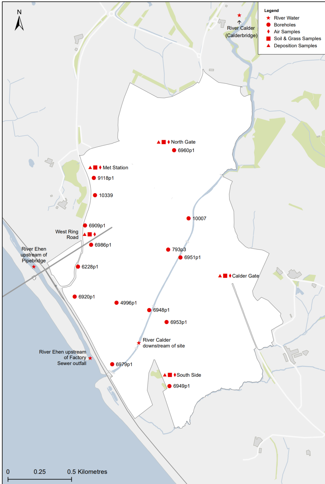
Figure 3. Terrestrial environmental monitoring at Sellafield
