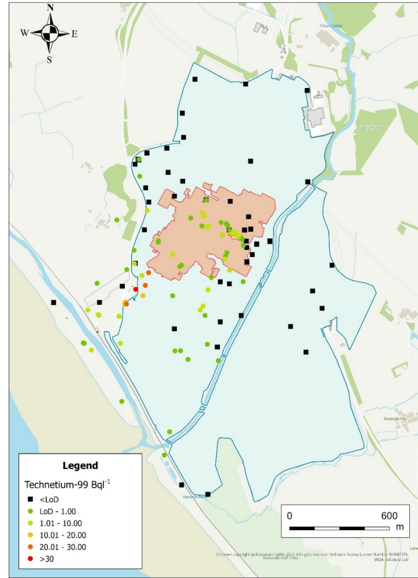
Figure 7. Average technetium-99 concentrations (Bq l -1 )
