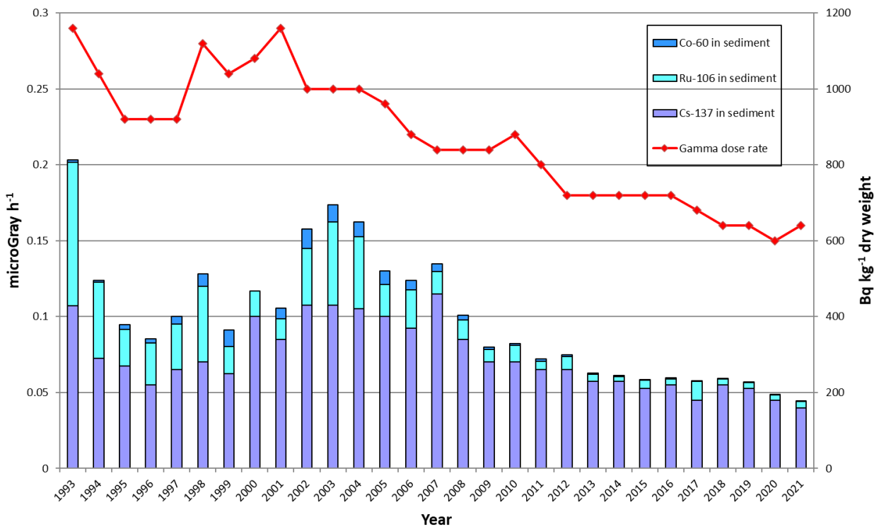
Figure B4. – External gamma dose rates at Newbiggin compared to sediment
