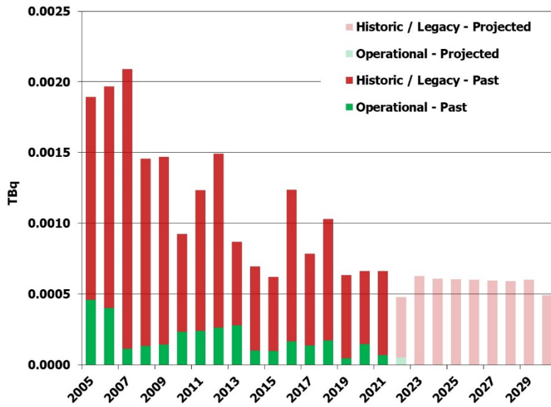
Figure 6. Past and projected tritium discharges from gaseous effluents
