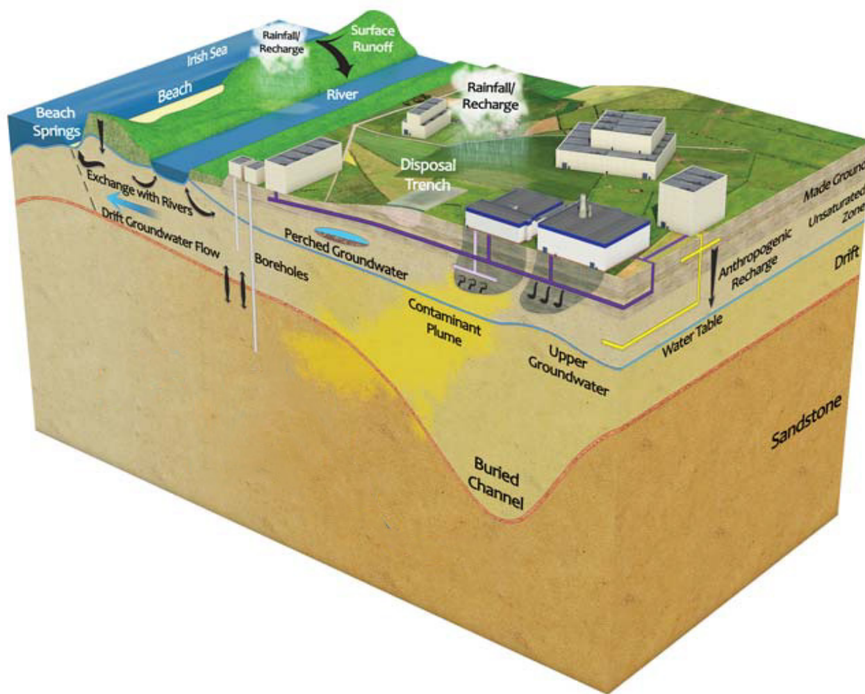
Figure 1. Schematic representation of Sellafield site geology and hydrogeology
