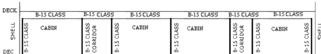
Figure 9.2 Fire integrity of bulkheads and ceilings in accommodation
