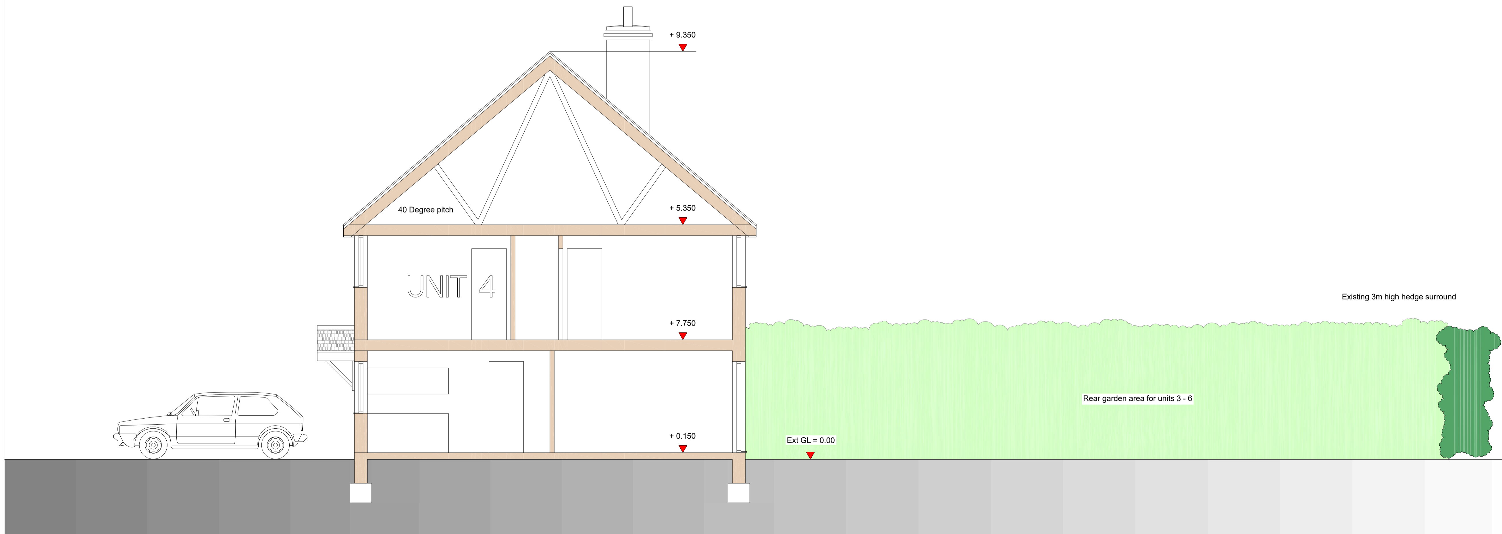
SECTION UNIT 3 - 6
