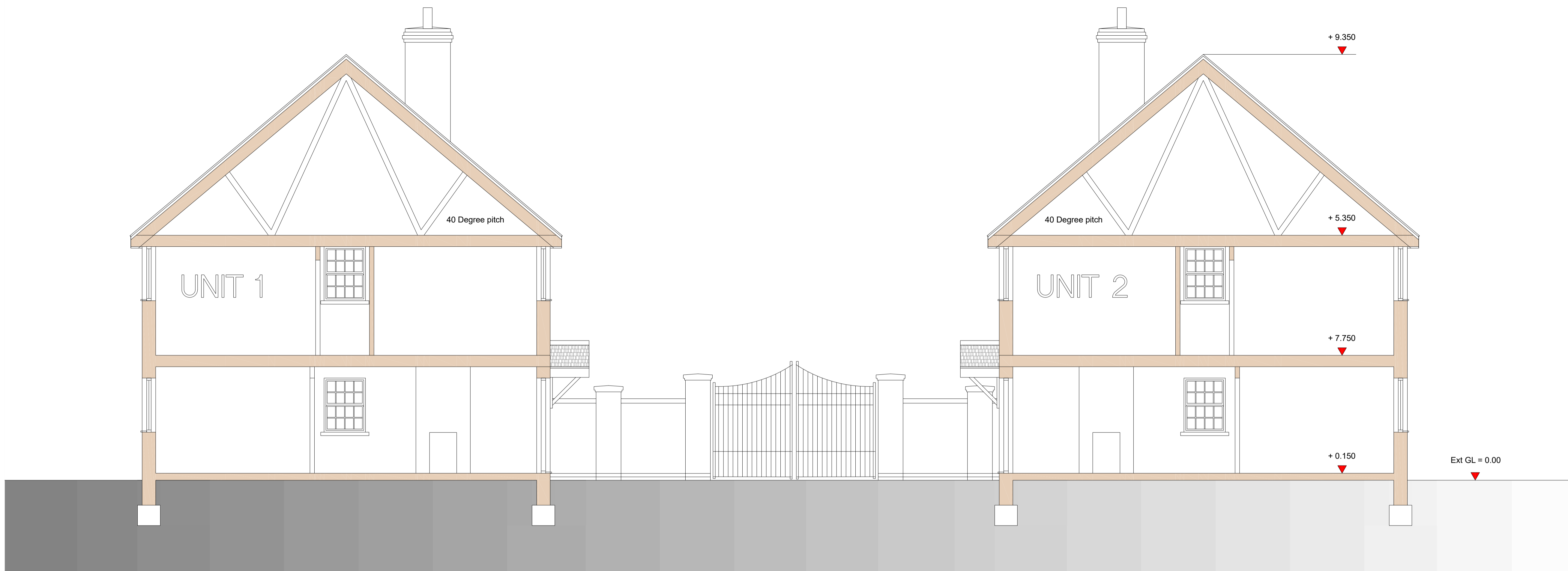
SECTION UNIT 1 - 2
