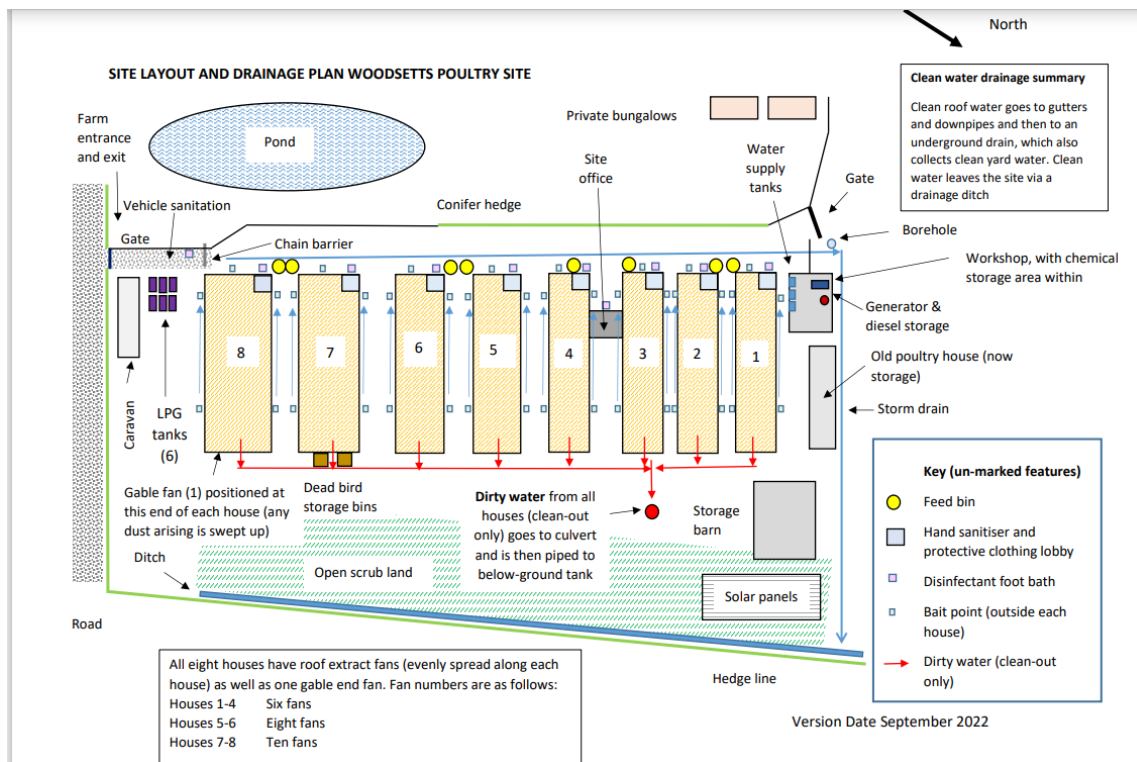
Site drainage plan
