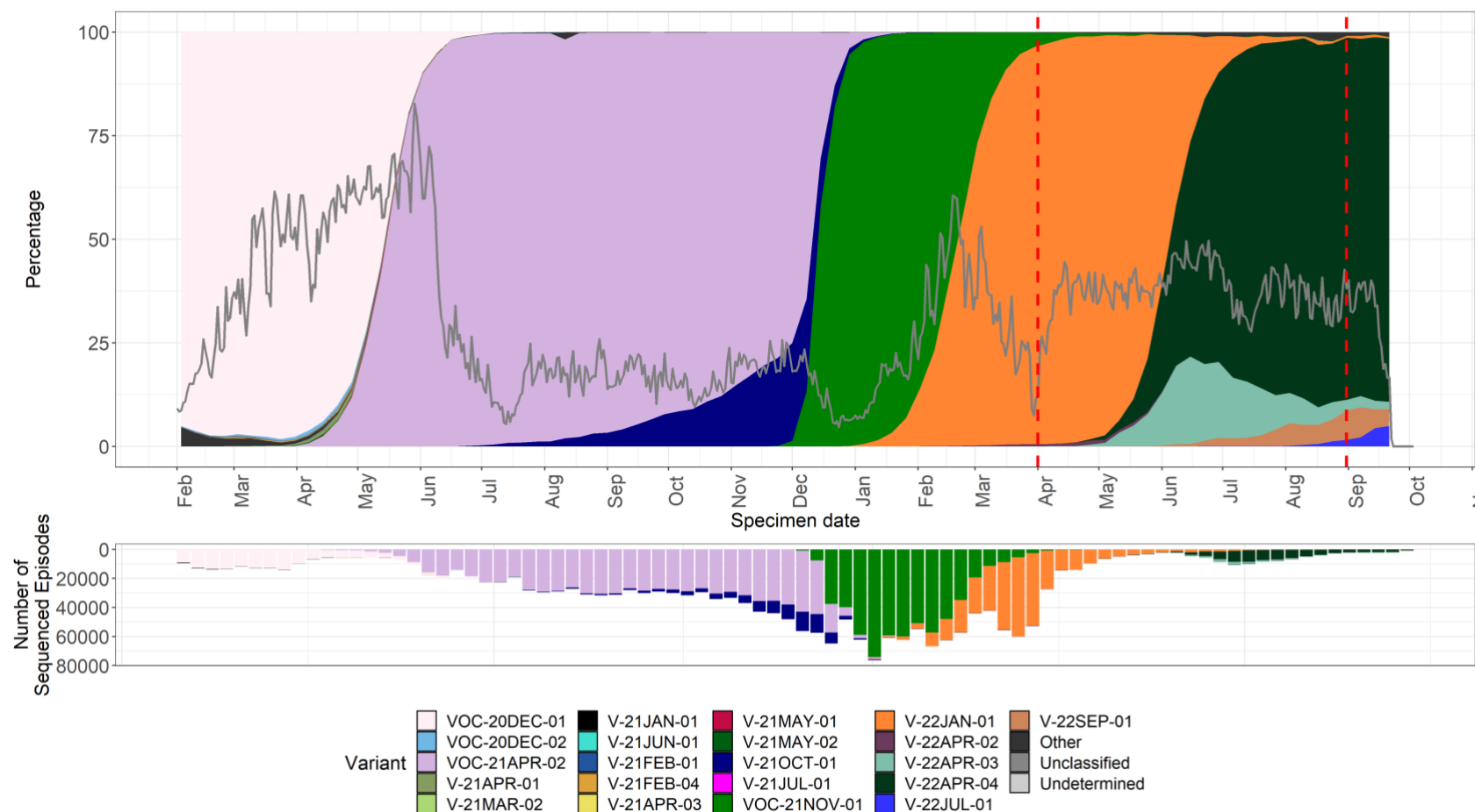
Figure 57. Prevalence of SARS-CoV-2 variants amongst available sequences episodes for England from 1 February, as of 04 October 2022
