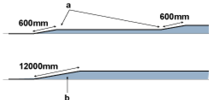
(Top) Successive 50mm ramps for shared surfaces (Bottom) Single 100mm ramp for shared surfaces
