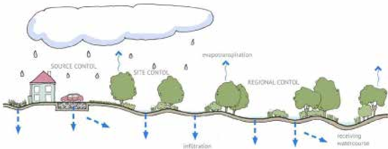
SuDS Management Train (from Susdrain, 2017)
