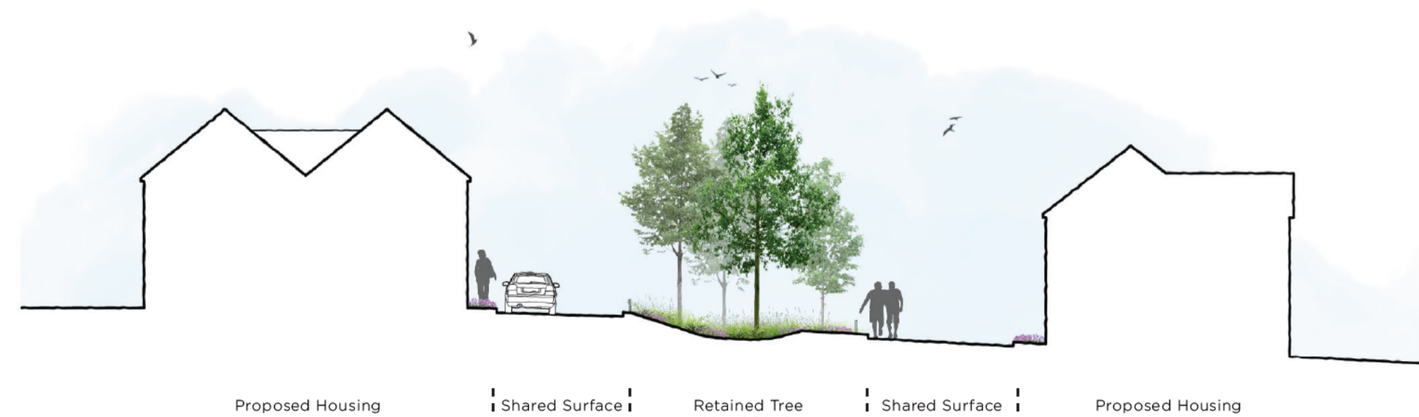
SITE SECTIONS E-E
